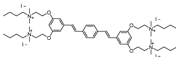
Formula G ("COE2-3C-C2butyl")
