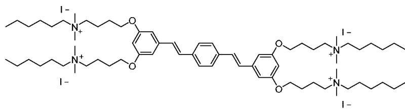
Formula T ("COE2-3C-C4hexyl")
