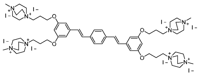
Formula DD ("COE2-3C-C3DABCO")
