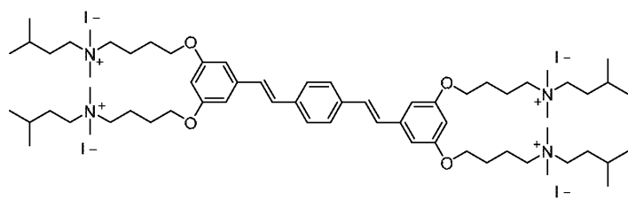
Formula U ("COE2-3C-C4isopentyl")
