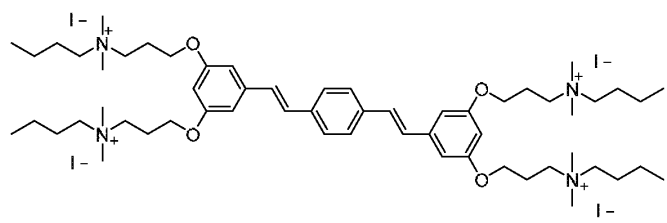
Formula AA ("COE2-3C-C3butyl")
