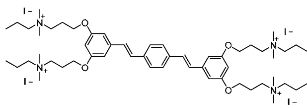
Formula Z ("COE2-3C-C3propyl")
