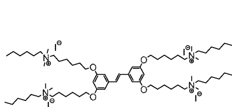
Formula E ("COE2-2hexyl")
