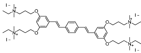
Formula Y ("COE2-3C-C3ethyl")
