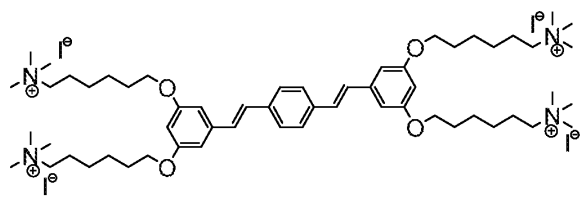
Formula O ("COE2-3C")
