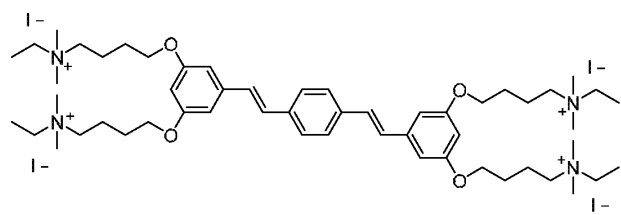
Formula P ("COE2-3C-C4ethyl")
