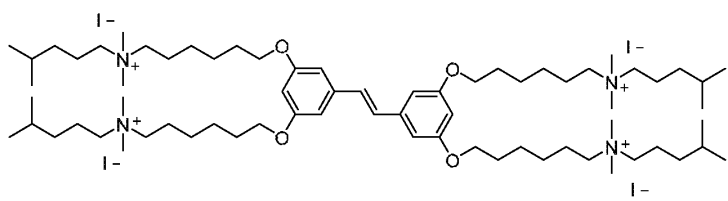
Formula L ("COE2-2isohexyl")
