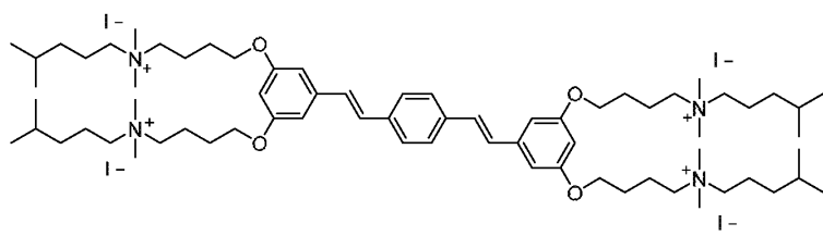
Formula V ("COE2-3C-C4isohexyl")
