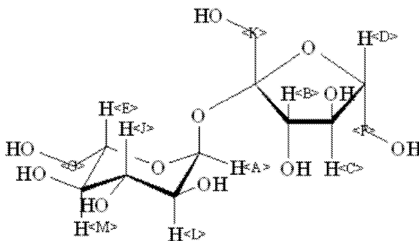
Formula (I)
