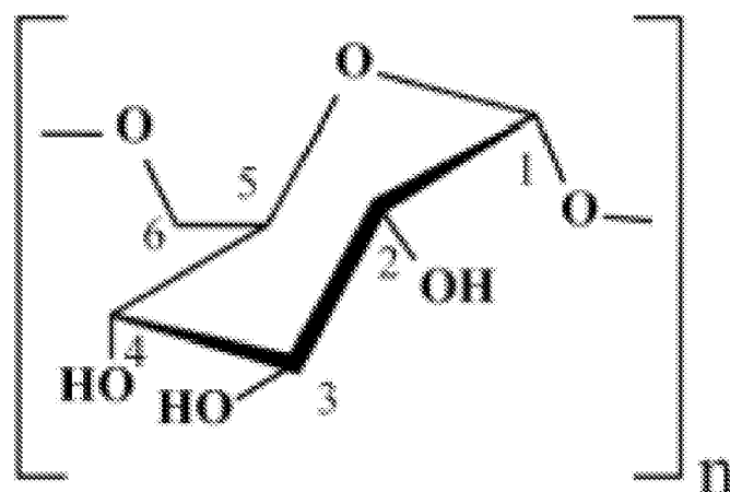
Dextran \alpha -(1-6)
