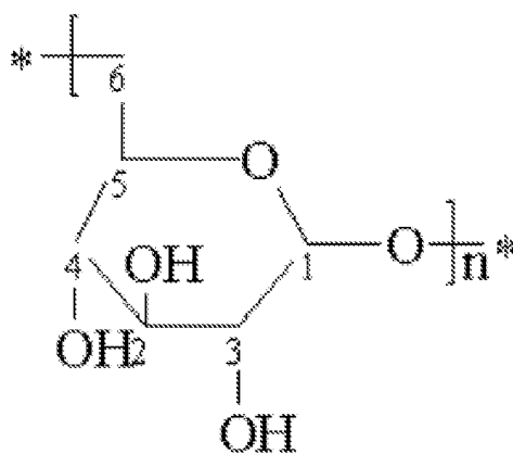
Formula (III)
