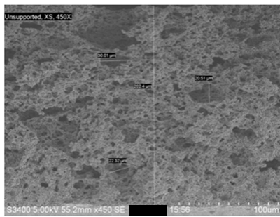
Cross-section SEM
