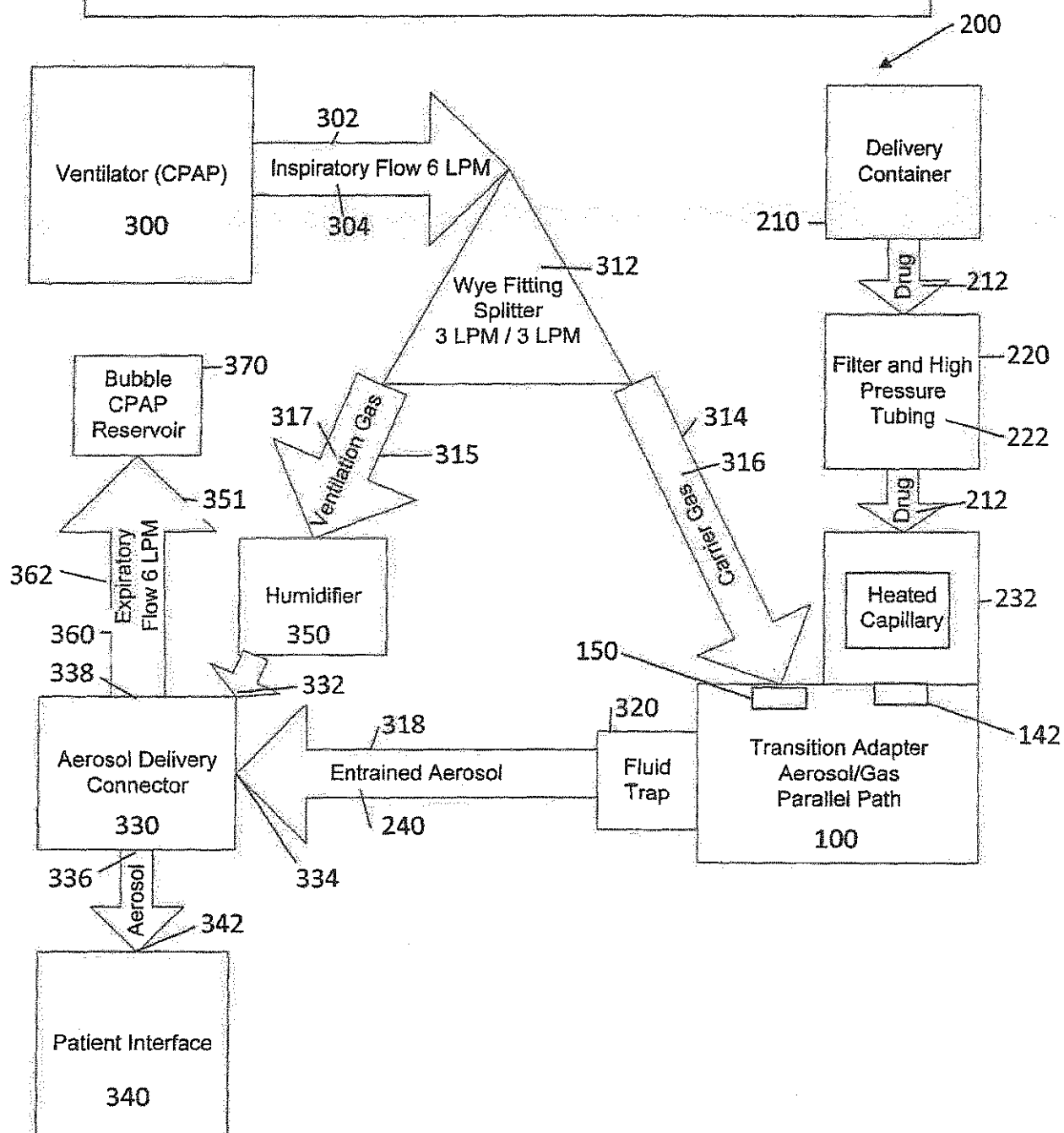
Fig. 7B: Bubble CPAP Ventilator Aerosol Delivery System
