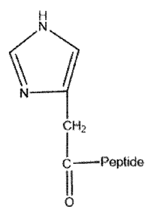
Imidazoacetyl (CA)-GLP-2
