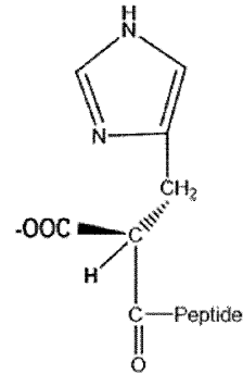
Beta-carboxyl-imidazopropionyl (CX)-GLP-2
