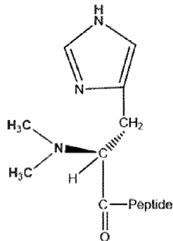
Dimethyl-histidyl (DM)-GLP-2
