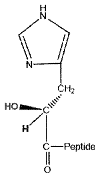
Beta-hydroxy-imidazopropionyl (HY)-GLP-2
