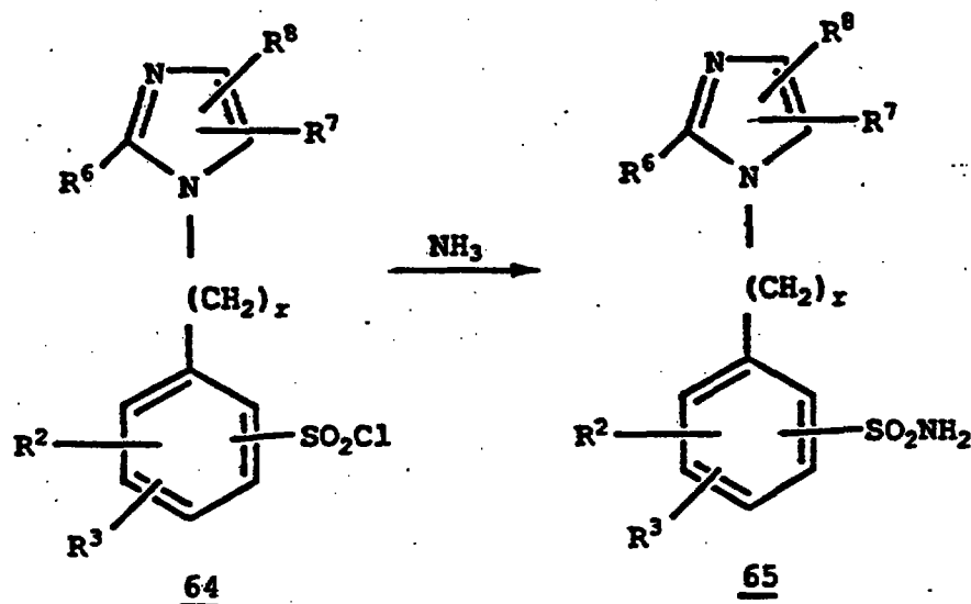
Scheme 10
