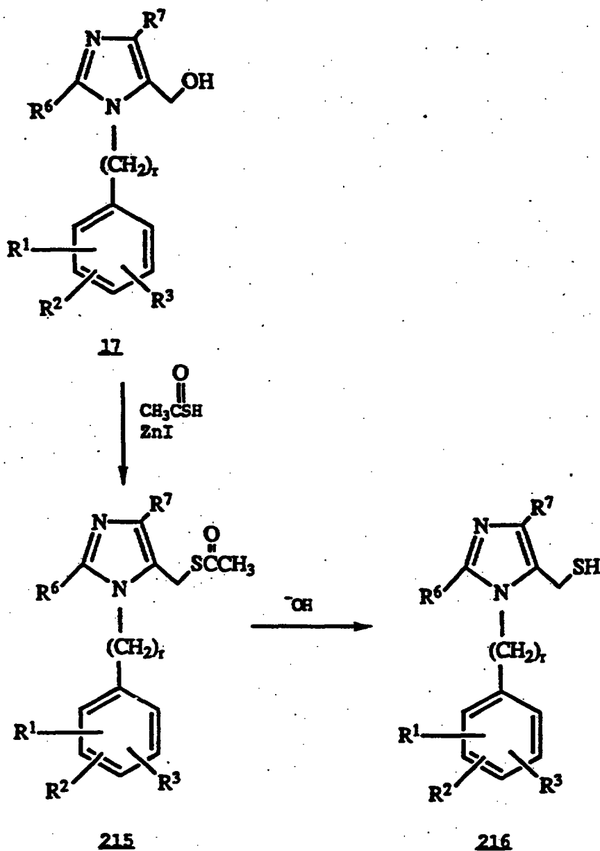
Scheme 32
