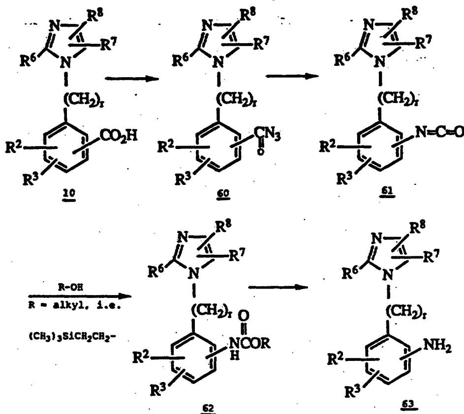
Scheme 9
