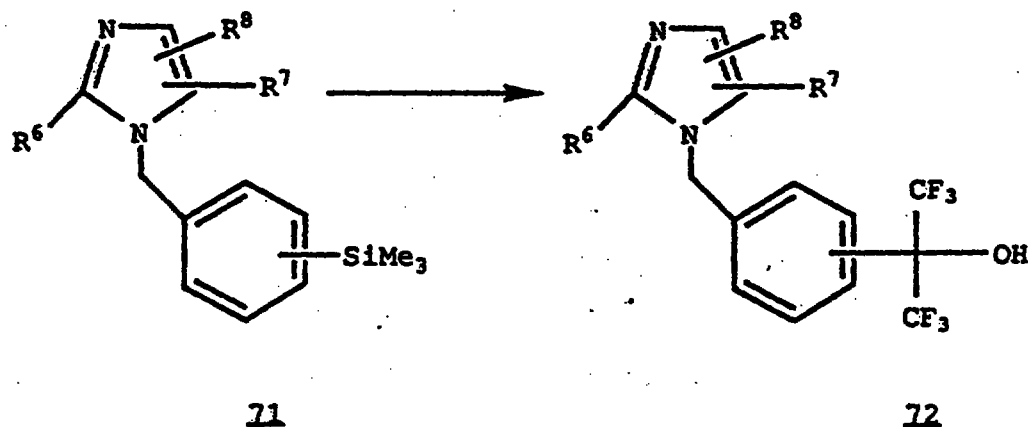
Scheme 12
