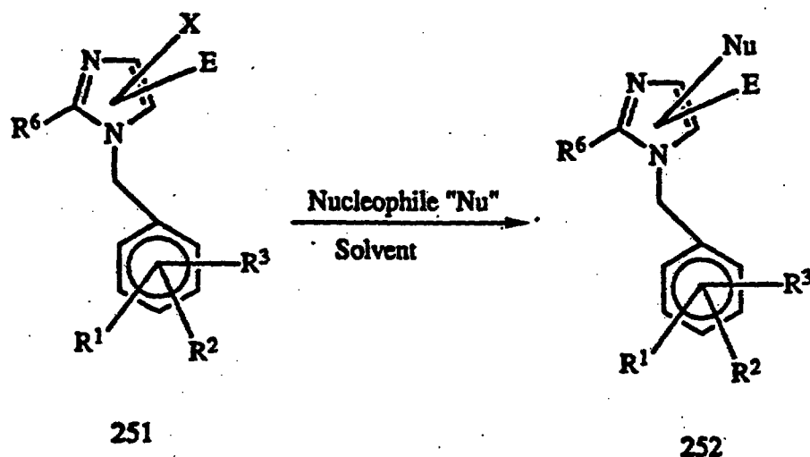
Scheme 40
