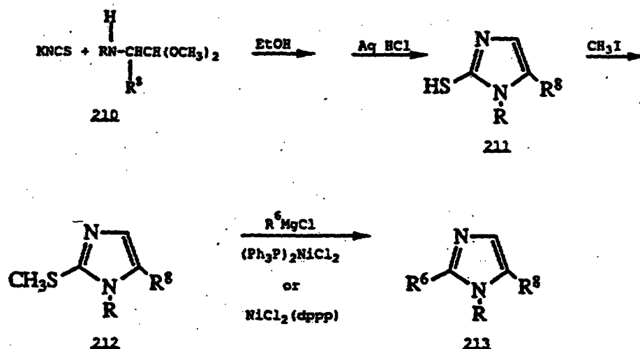
Scheme 31
