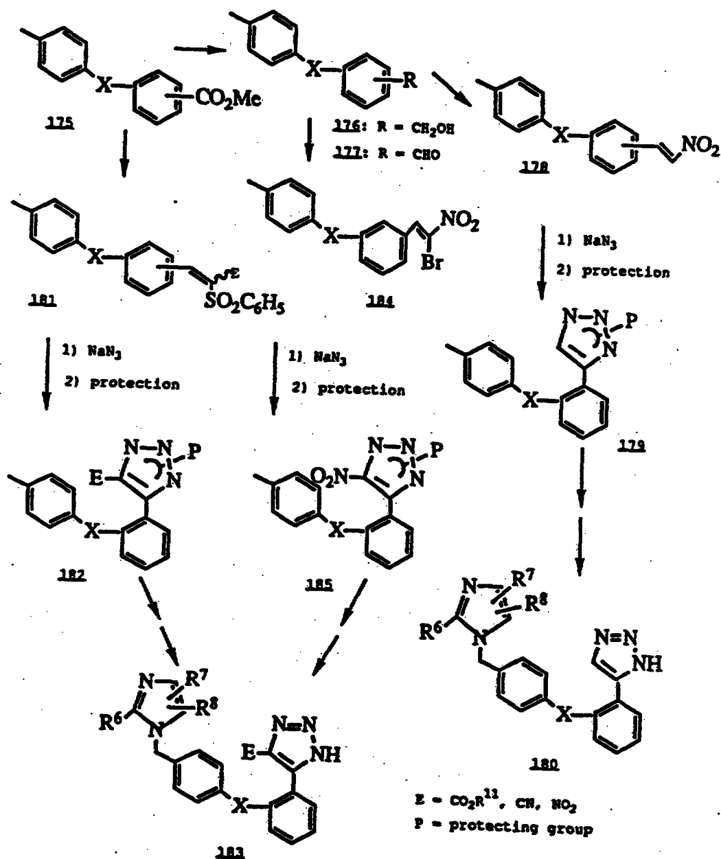
Scheme 26
