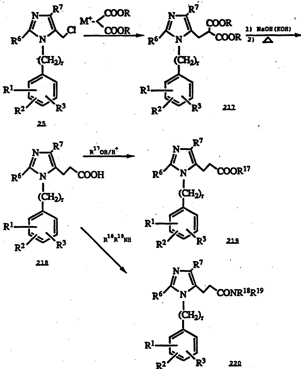
Scheme 33
