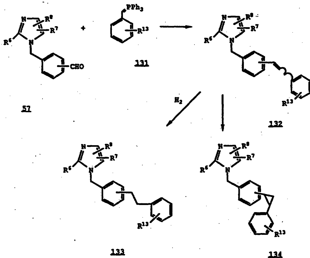
Scheme 20
