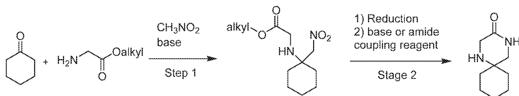
Scheme 6. General preparation of 1,4-diazaspiro[5.5]undecan-3-one with only two isolations.
