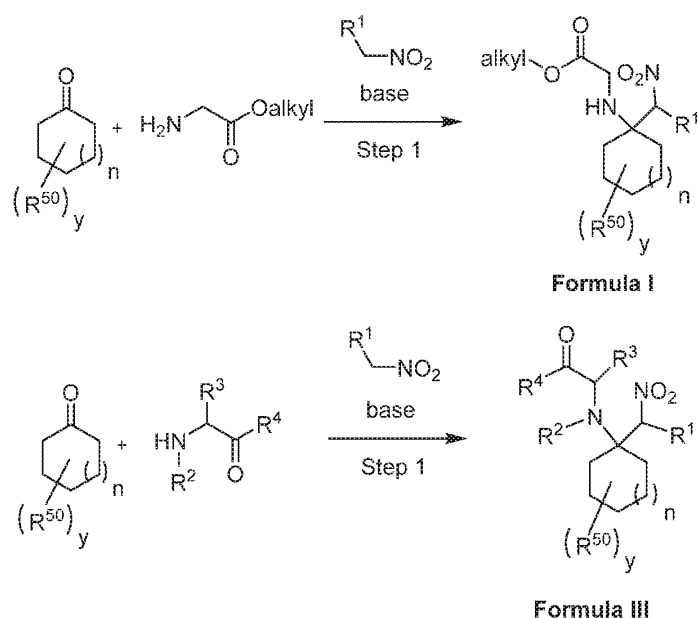
Scheme 10. Synthesis of Compounds of Formula I and Formula III
