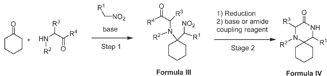
Scheme 9. Additional preparation of compounds of Formula IV with only two isolation steps.
