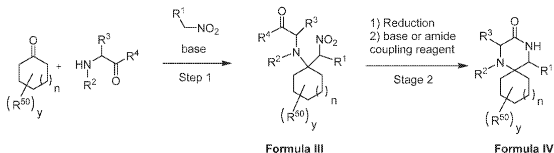
Scheme 8. General preparation of compounds of Formula IV with only two isolation steps.
