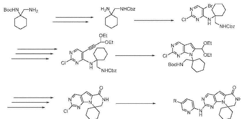
Scheme 1. Prior synthesis of N-(heteroaryl)-pyrrolo[3,2-d]pyrimidin-2-amine cyclin dependent kinase inhibitors.
