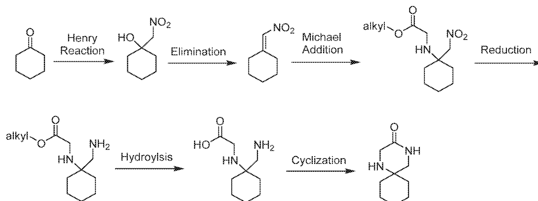
Scheme 3. Improved synthetic route to prepare 1,4-diazaspiro[5.5]undecan-3-one.
