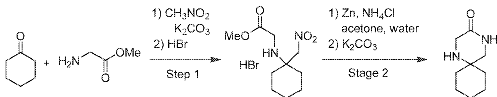
Scheme 5. Utilization of hydrobromic acid to isolate the Michael addition product.
