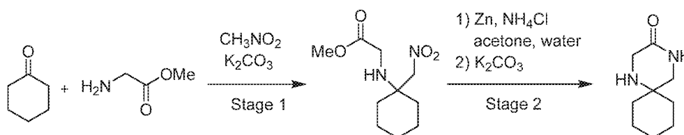
Scheme 4. Preparation of 1,4-diazaspiro[5.5]undecan-3-one with only two isolations.
