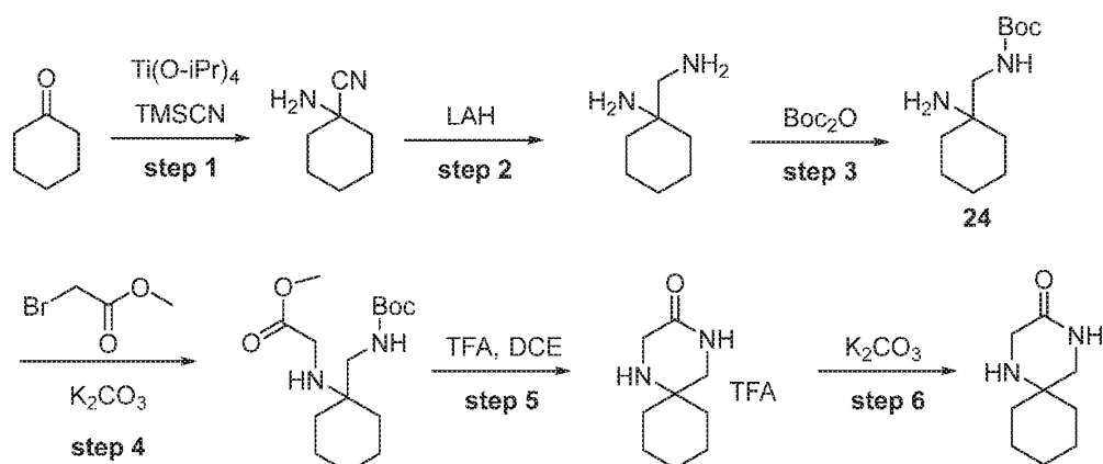
Scheme 2. Prior synthesis of 1,4-diazaspiro[5.5]undecan-3-one.
