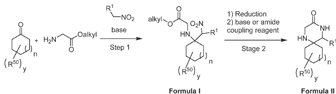
Scheme 7. General preparation of 1,4-diazaspiro[5.5]undecan-3-one with only two isolation steps.
