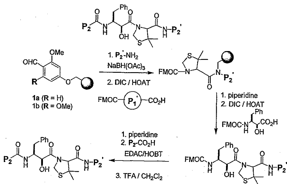
Scheme 3: Solid Phase Synthesis Of HIV Protease Inhibitors
