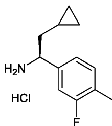
Compound 5-A
