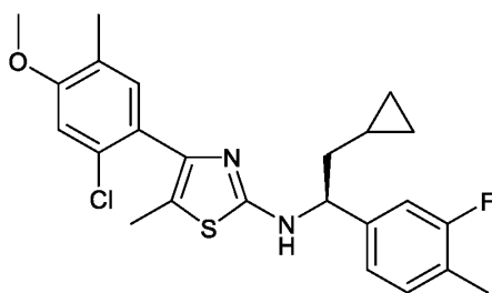
Compound 7-A
