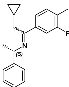
Compound 3-A
