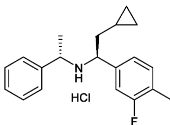
Compound 4-A
