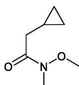
Compound 2-B
