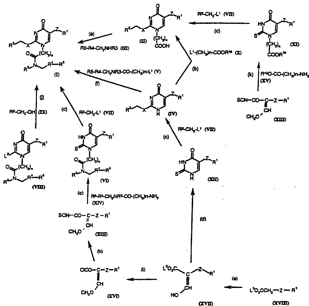
Scheme I
