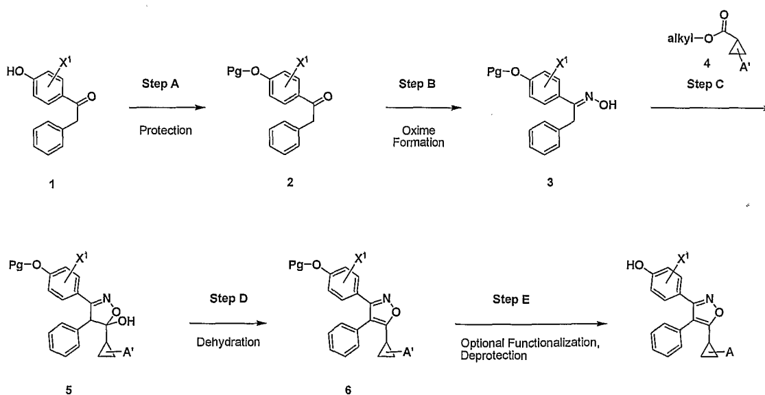
Scheme I. General Preparation of Isoxazoles
