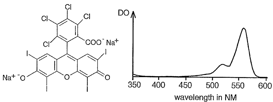
rose bengale
