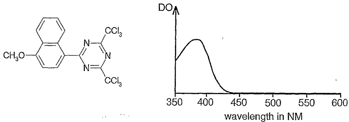
2-(4'-methoxy-1'-naphthyl)-4,6-bis(trichloromethyl)-1,3,5-triazine
