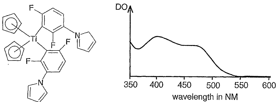
Irgacure 784
