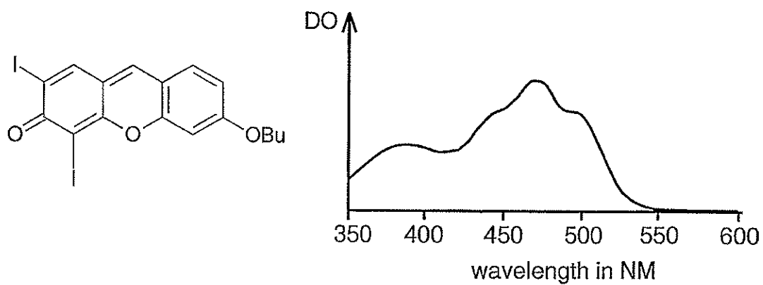
3-butoxy-5,7-diiodo-6-fluorone
