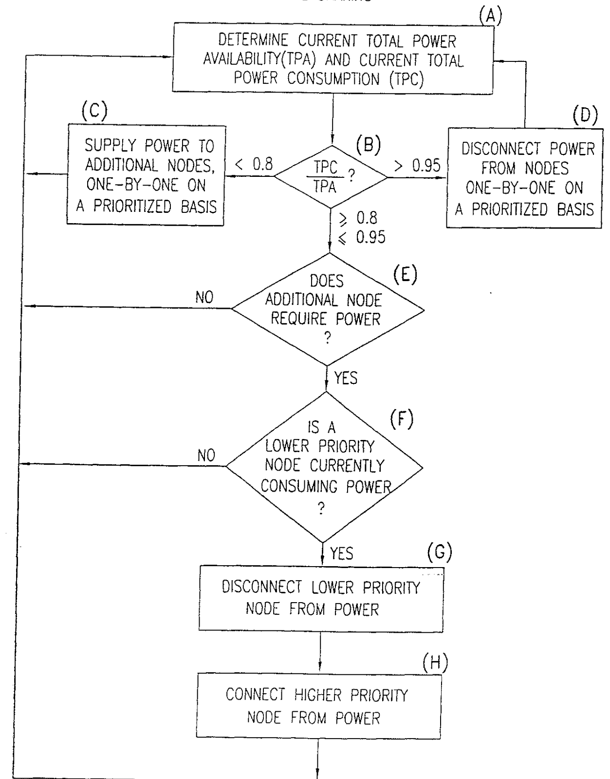
FIG. 19D INVOLUNTARY POWER MANAGEMENT FULL FUNCTIONALITY OR NO FUNCTIONALITY TIME SHARING
