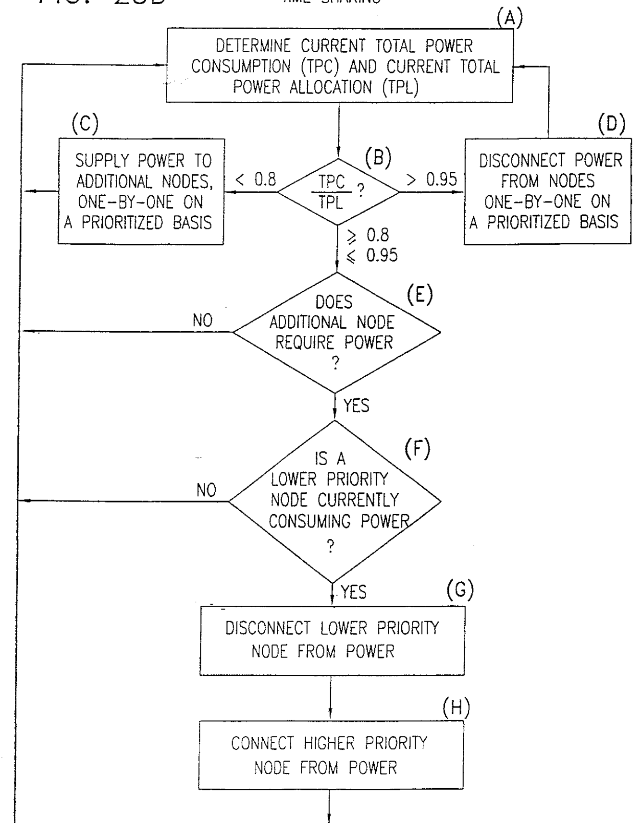
FIG. 23D VOLUNTARY POWER MANAGEMENT FULL FUNCTIONALITY OR NO FUNCTIONALITY TIME SHARING
