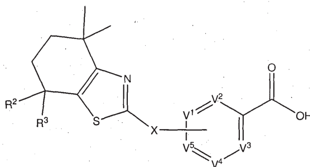
Formula (IIa)
