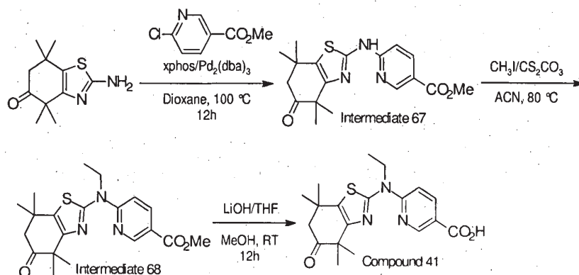
Scheme 19
