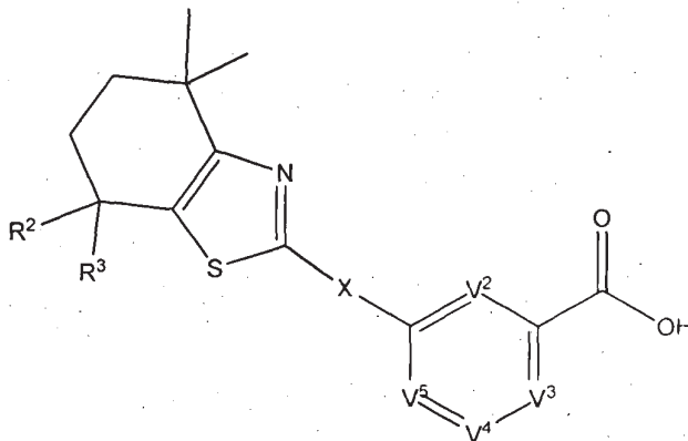
Formula (IIIa)
