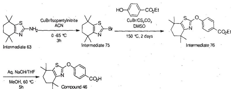
Scheme 23
