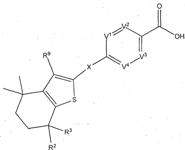
Formula (IIId)
