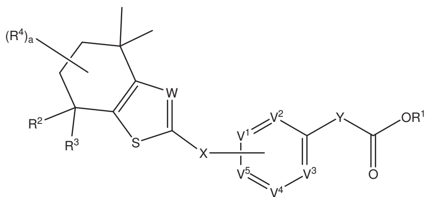
Formula (I)
