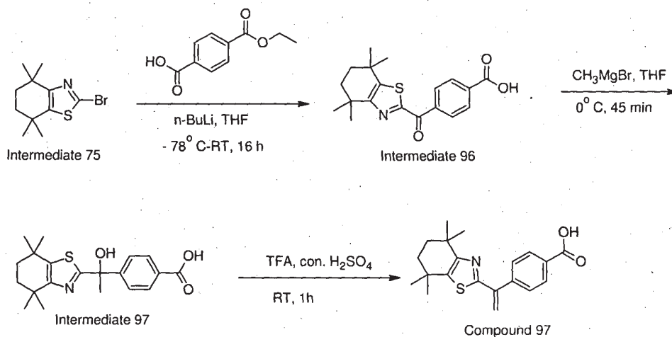
Scheme 44
