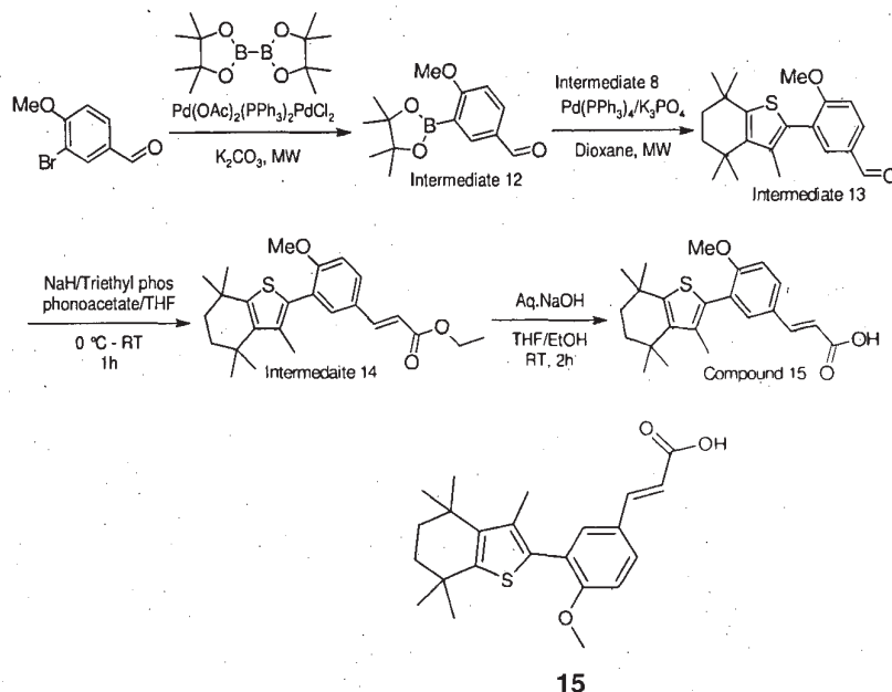
Scheme 7
