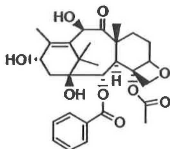
formula (XI).
