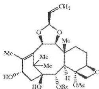
formula (III)
