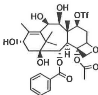
formula (X).
