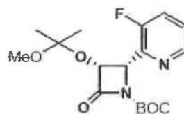
formula (VI)
