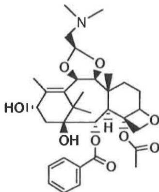
formula (Ia)
