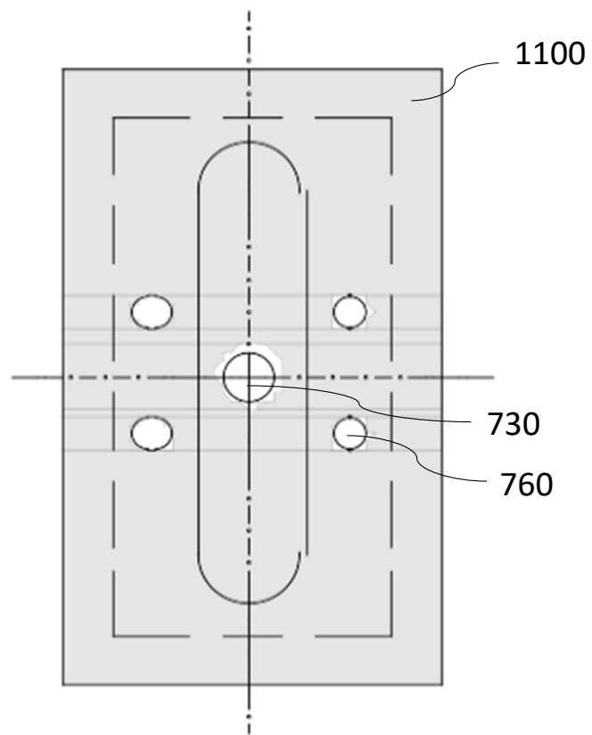
CAPPING PLATE
