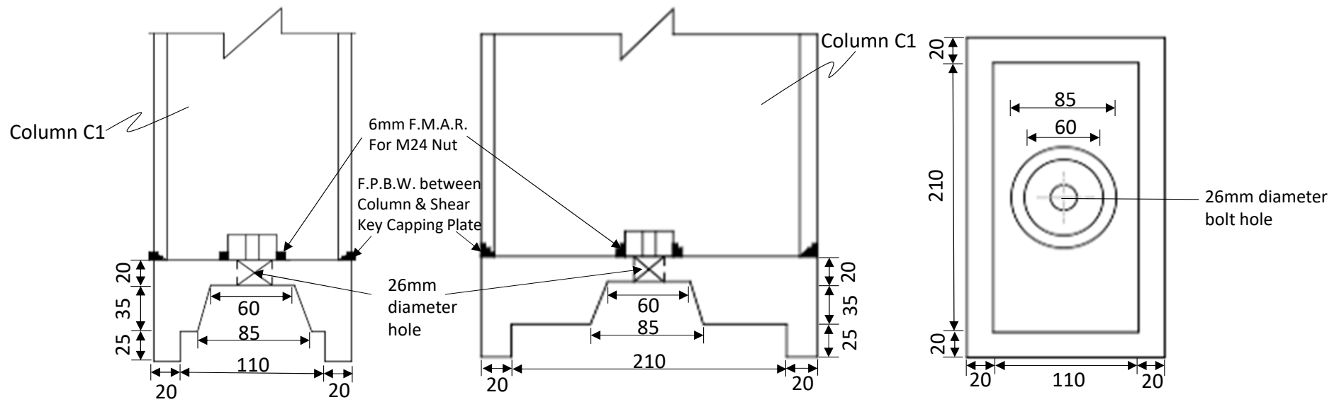
TYPE 1 COLUMN SPLICE BASE
