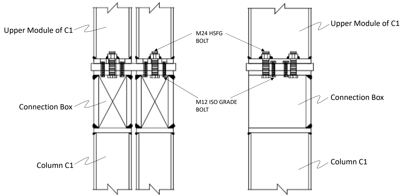
TYPE 2 COLUMN JOINT
