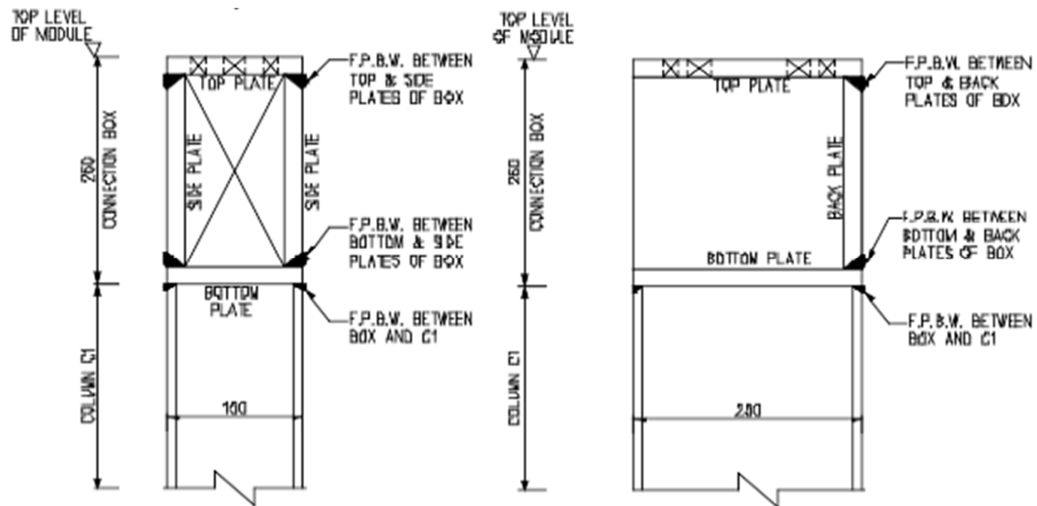
TYPE 2 COLUMN SPLICE
