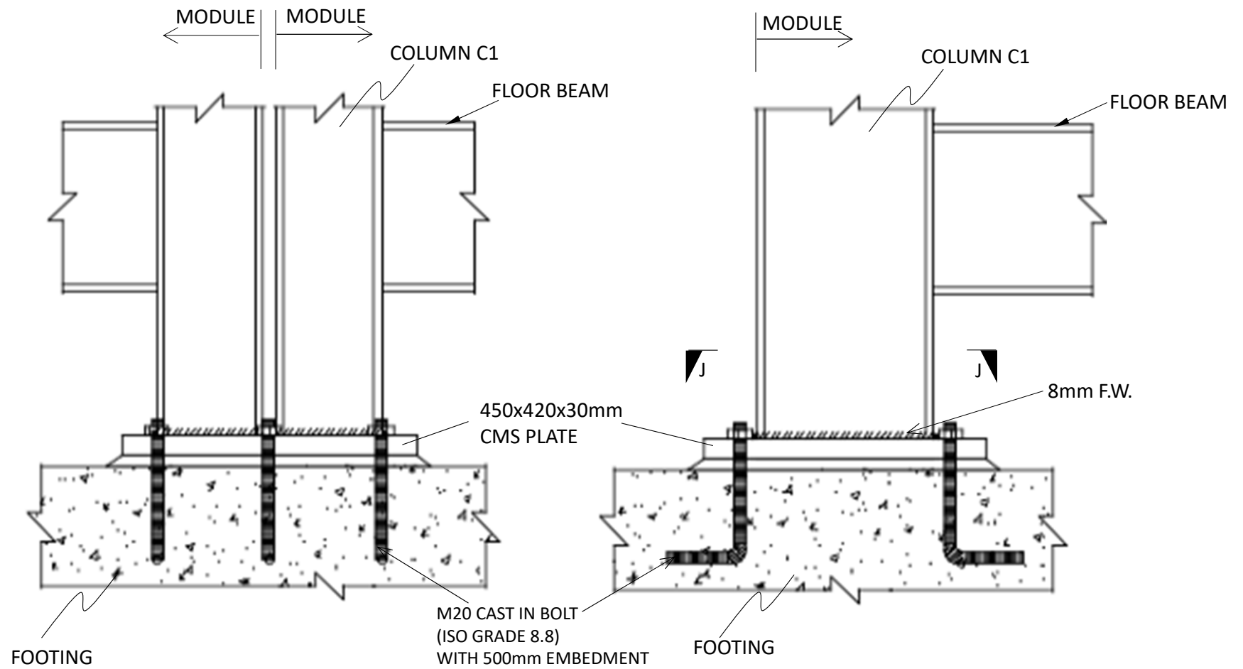
BASE FIXING FOR INTERIOR COLUMN TO FOOTINGS
