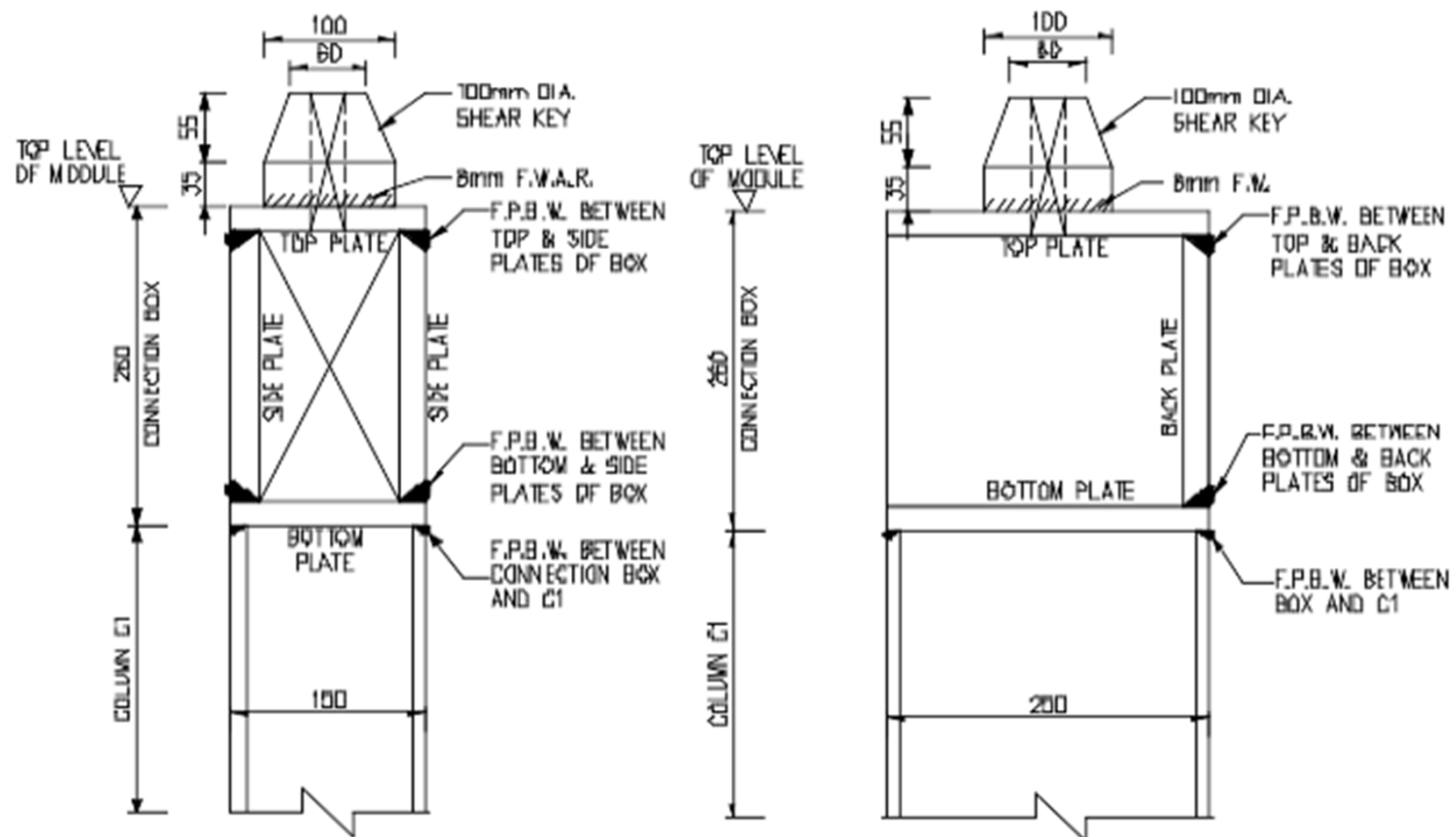
TYPE 1 COLUMN SPLICE
