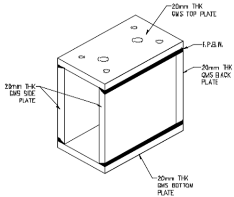
ISOMETRIC VIEW OF CONNECTION BOX FOR TYPE 2 COLUMN SPLICE
