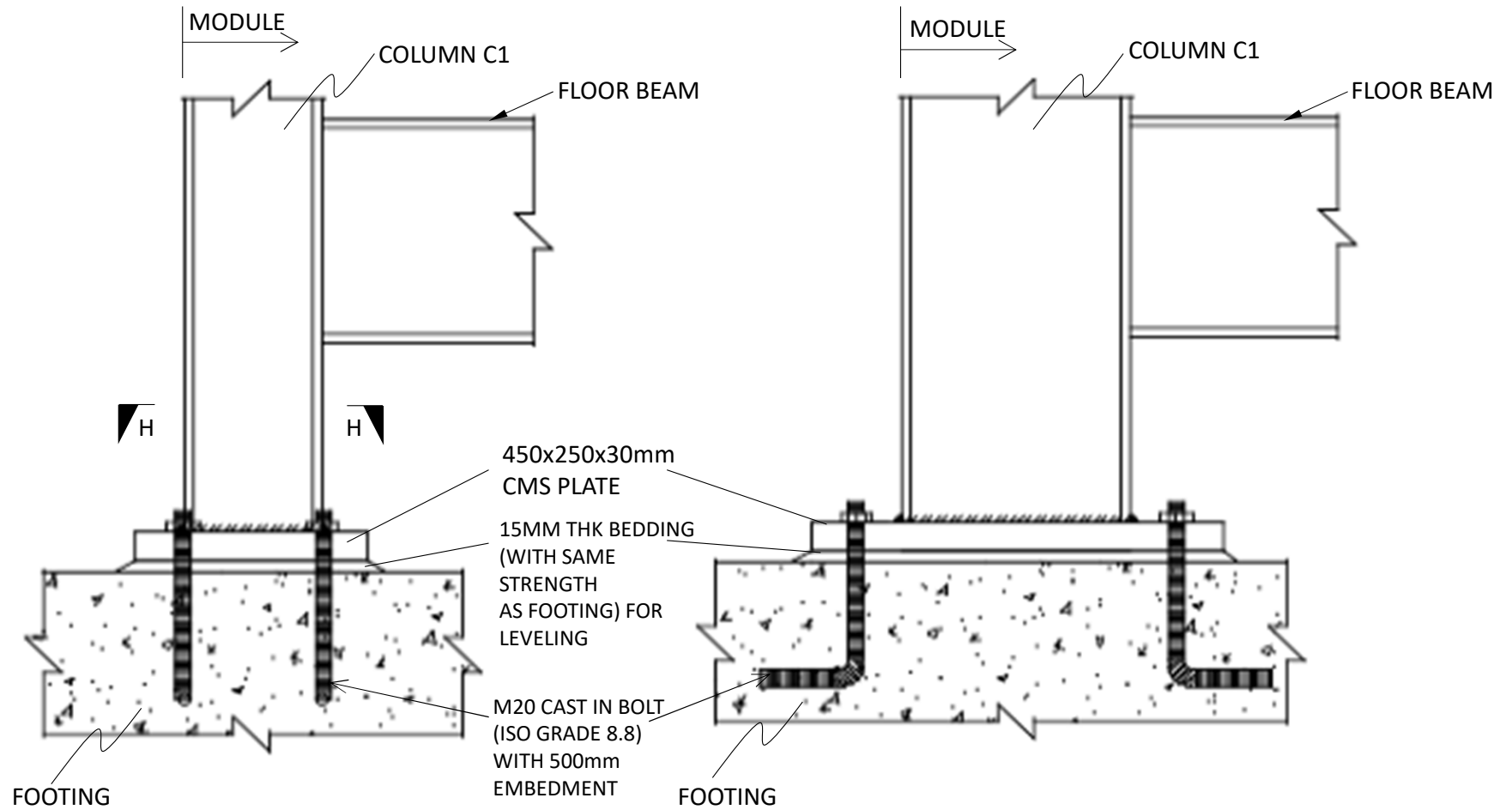
BASE FIXING FOR EDGE COLUMN TO FOOTINGS
