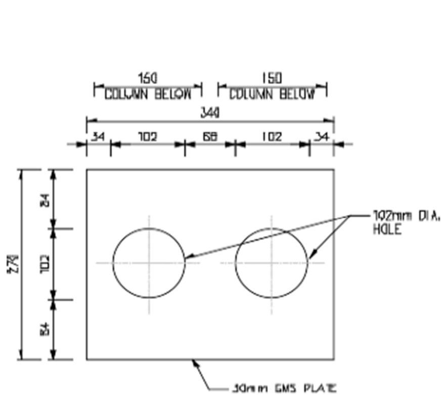
CONNECTING PLATE
