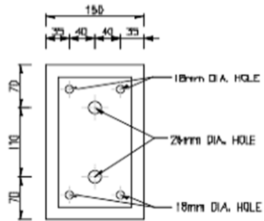
TOP VIEW OF CONNECTION BOX TOP PLATE
