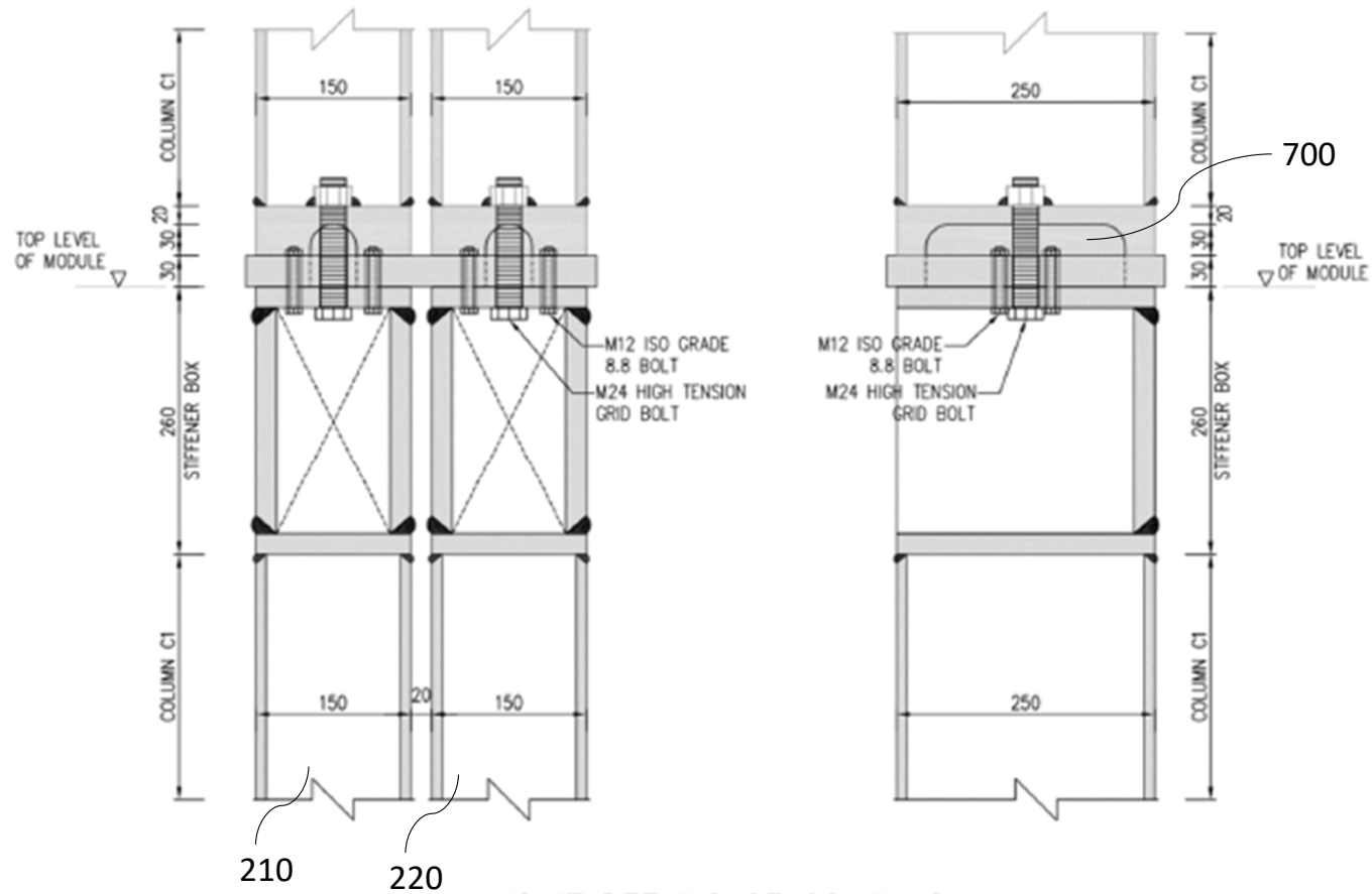
JOINT DETAILS OF COLUMNS
