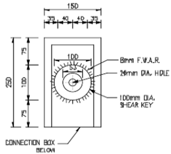
TOP VIEW OF CONNECTION BOX TOP PLATE
