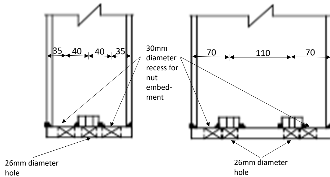
TYPE 2 COLUMN SPLICE BASE
