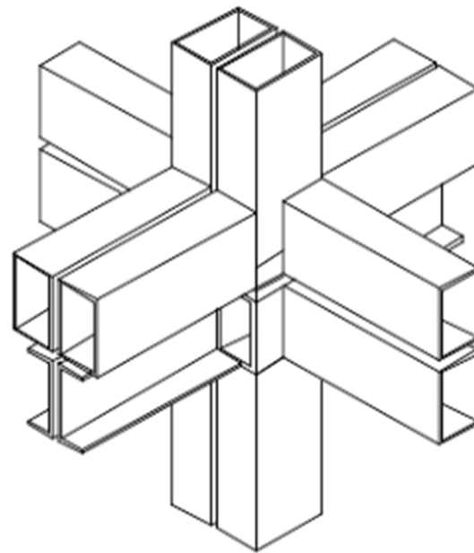
ISOMETRIC VIEW OF TYPE 1 COLUMN SPLICE JOINT
