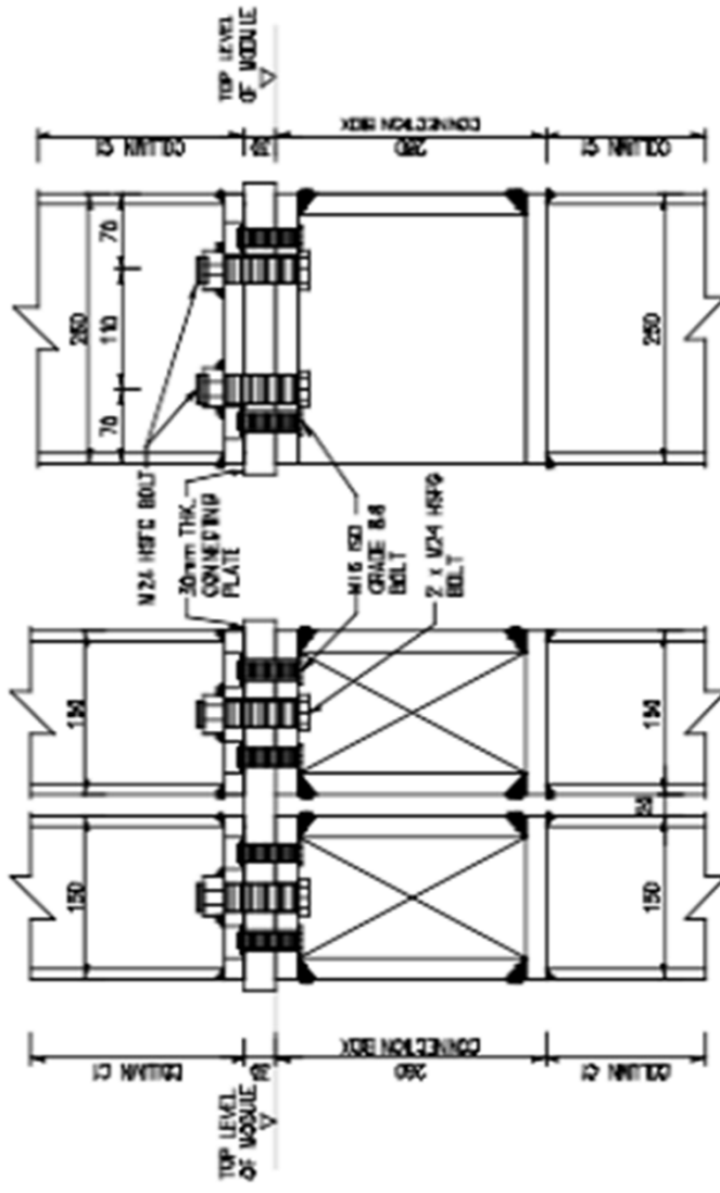
TYPE 2 COLUMN SPLICE
