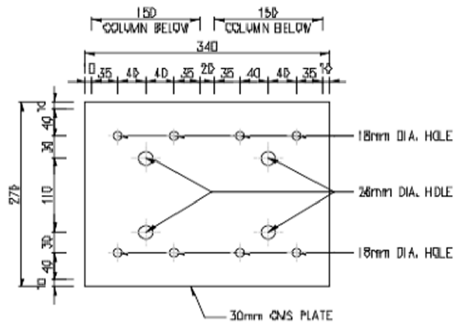
CONNECTING PLATE
