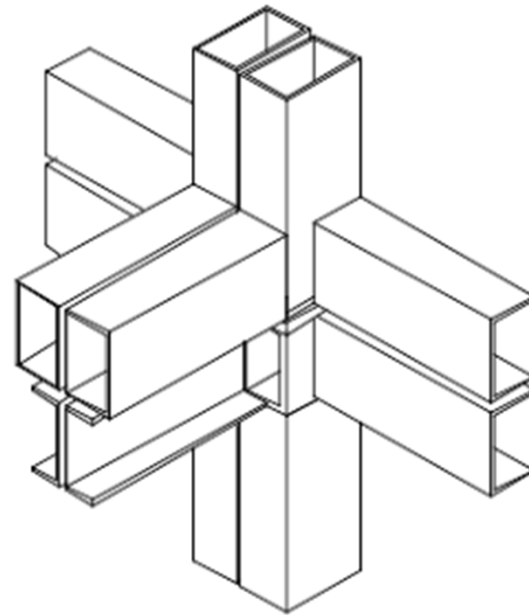
ISOMETRIC VIEW OF TYPE 2 COLUMN SPLICE JOINT
