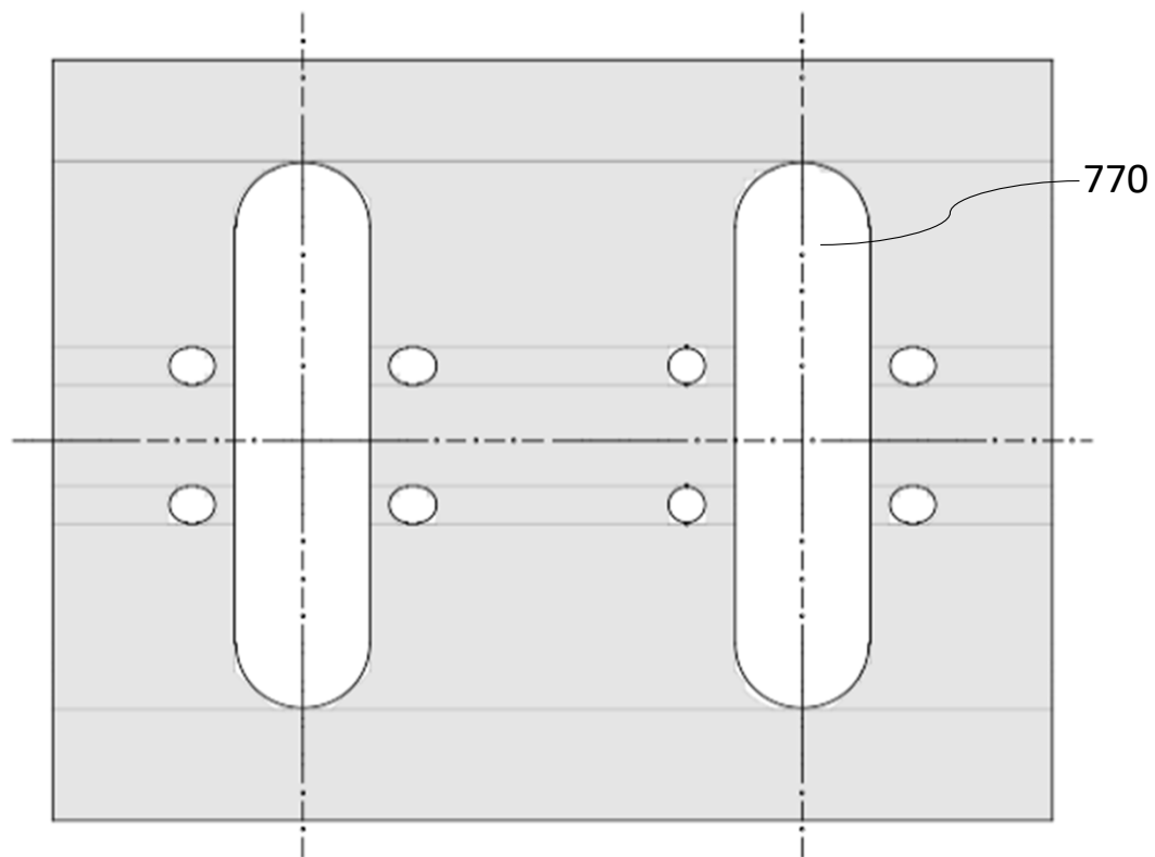
CONNECTING PLATE
