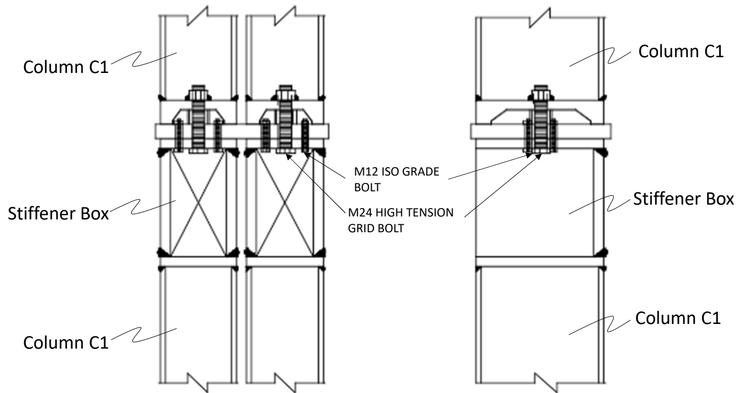
TYPE 1 COLUMN JOINT
