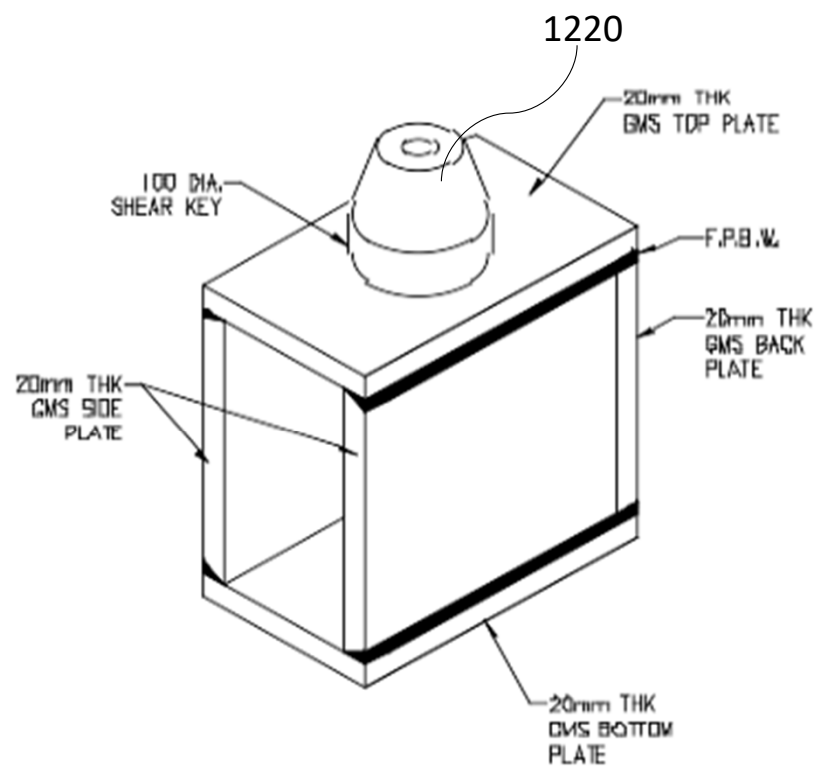
ISOMETRIC VIEW OF CONNECTION BOX FOR TYPE 1 COLUMN SPLICE
