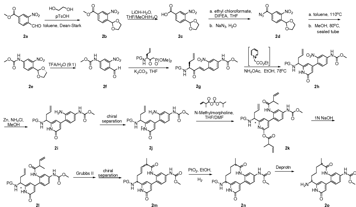
Scheme 2
