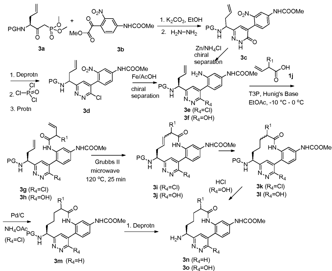
Scheme 3
