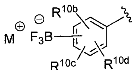
R 4 -5 fluoride adduct
