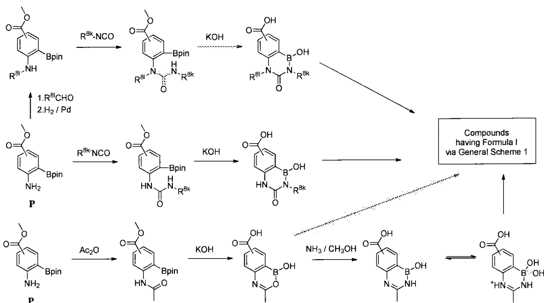
General Scheme 8
