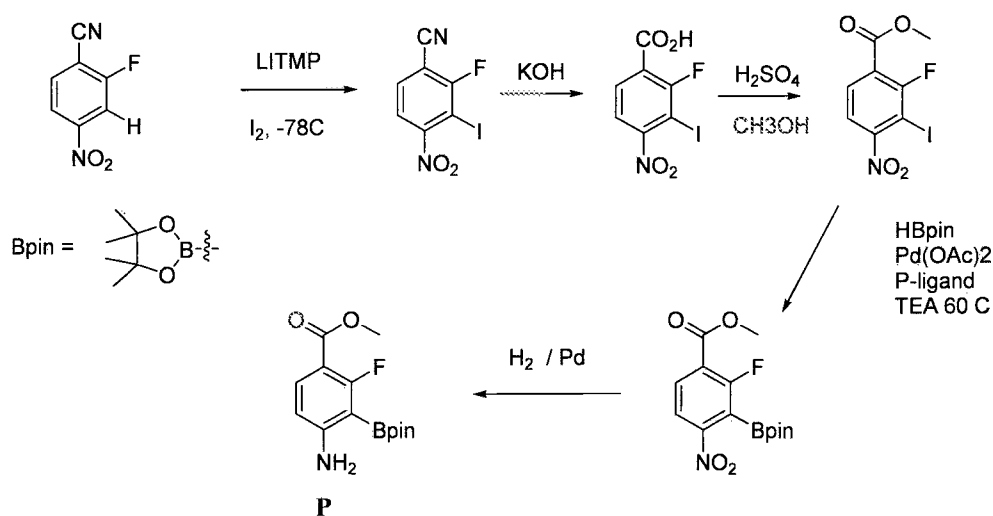
General Scheme 7
