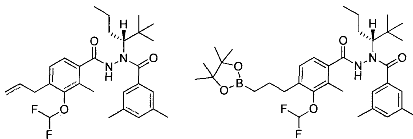
SKC-04-052 (mixture, 36:62 ratio)
