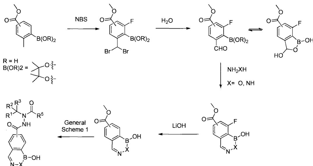
General Scheme 5
