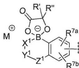
\text{R}^4 -1 hydroxy acid adduct
