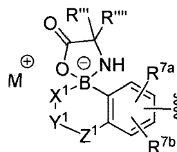
R^4 -1 amino acid adduct
