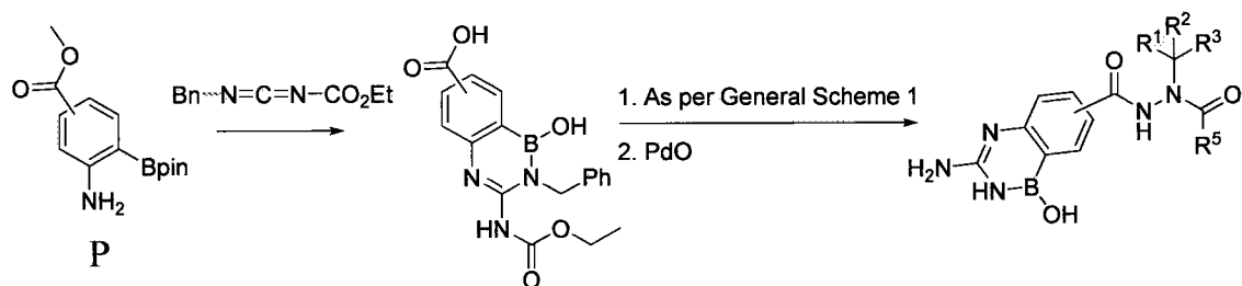
General Scheme 8
