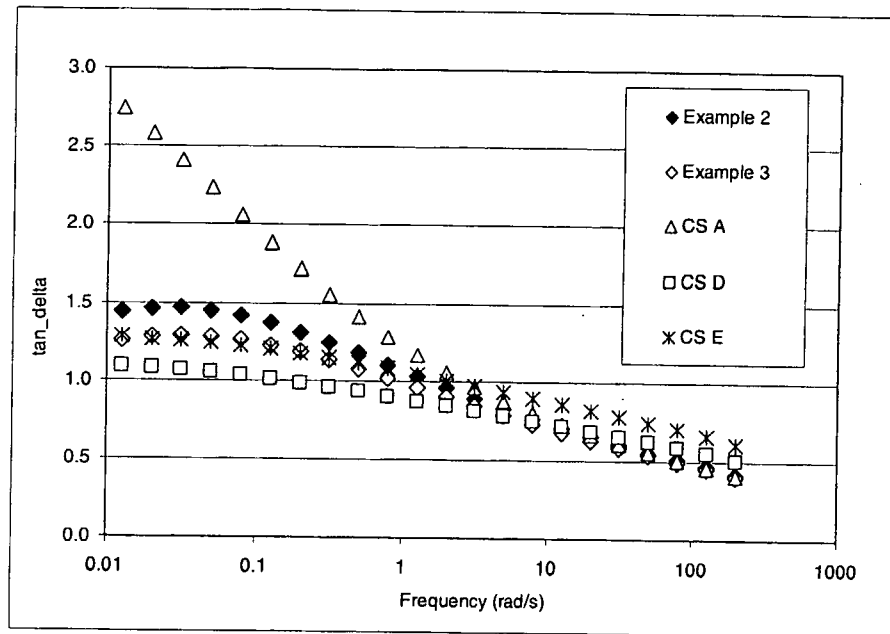
FIG. 3 Tan Delta Comparison
