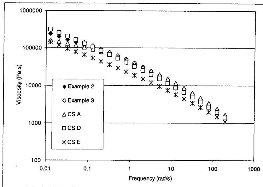
FIG. 2 Low Shear Viscosity Comparison
