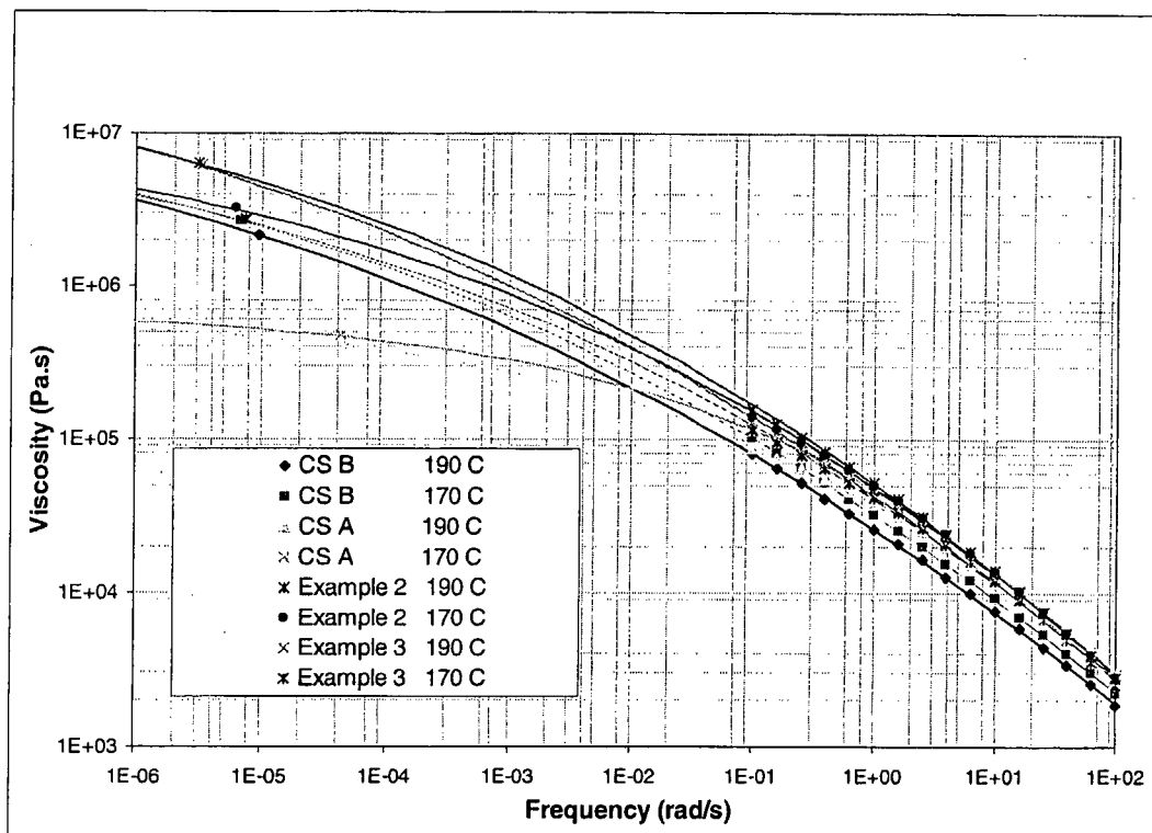
Figure 1: Low Shear Viscosity Characterization of Inventive and Comparative Example Samples
