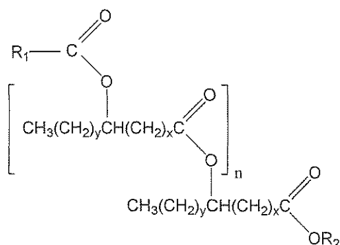
Formula V
