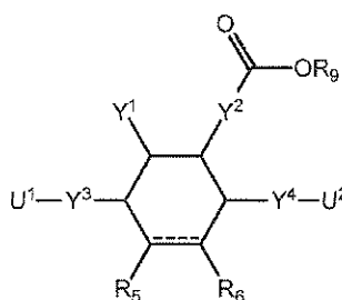
Formula II
