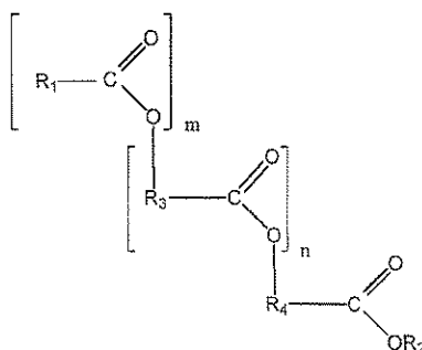
Formula IV
