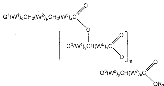
Formula III
