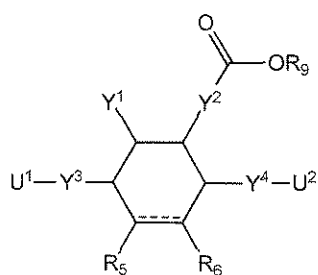
Formula II
