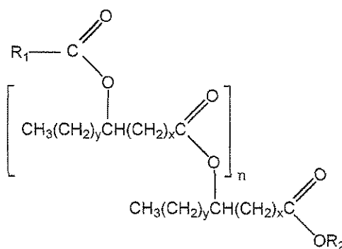
Formula V
