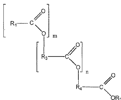
Formula IV
