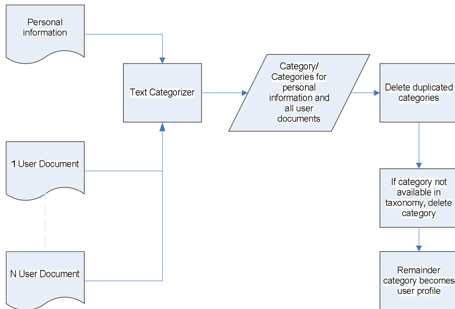
Figure B-2: process flow of matching category/categories between user profile and documents
