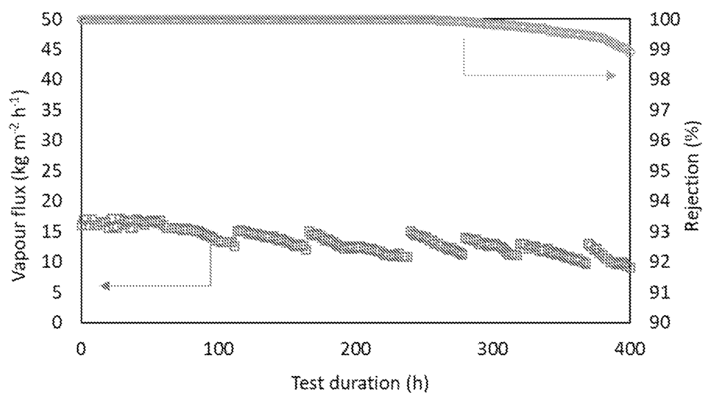
Figure 23
