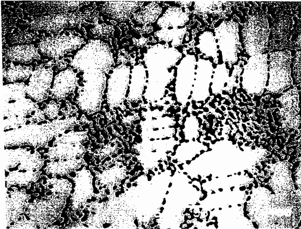
Figure 10. SEM backscattered image of the as-cast Co-(8 at. %)Cr-(7 at. %)Pt-(8 at. %)B alloy.
