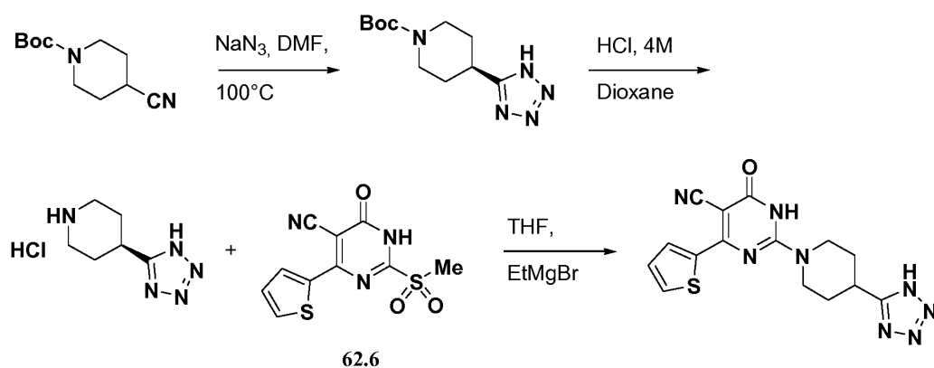
General Scheme J, 6-Oxo-2-[3-(1H-tetrazol-5-yl)-azetidin-1-yl]-4-thiophen-2-yl-1,6-dihydropyrimidine-5-carbonitrile
