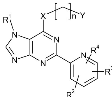
(VIb)
