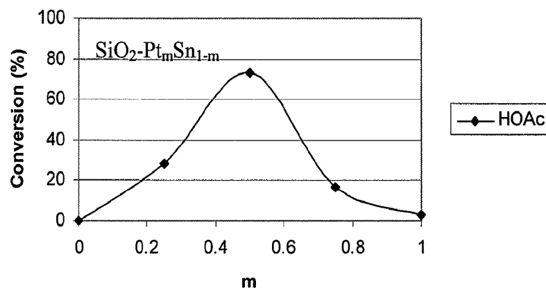
FIG. 1C - Conversion of HOAc
