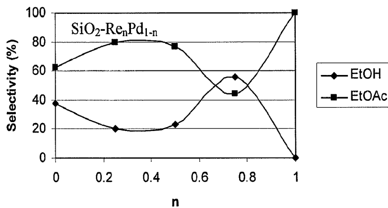
FIG. 2A - Selectivity of Re/Pd
