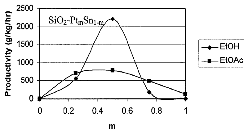
FIG. 1B - Productivity of Pt/Sn Catalyst
