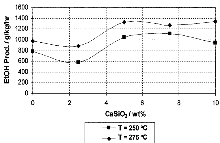
FIG. 6B - Productivity
