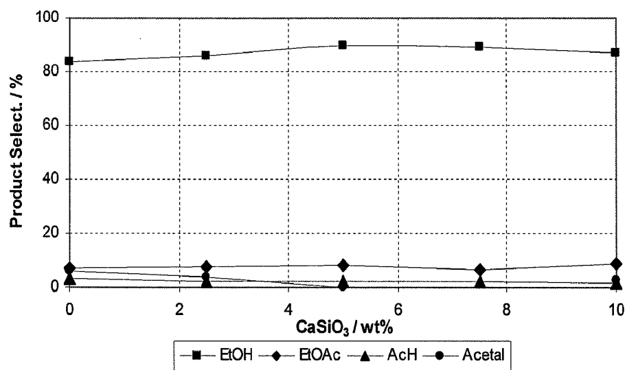
FIG. 6C - Selectivity @ 250
