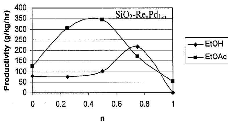
FIG. 2B - Productivity of Re/Pd
