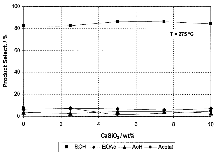
FIG. 6D - Selectivity @ 275
