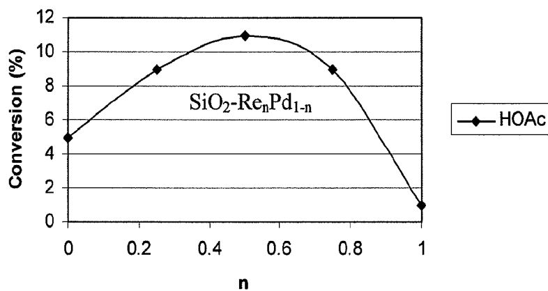
FIG. 2C - Conversion of HOAc
