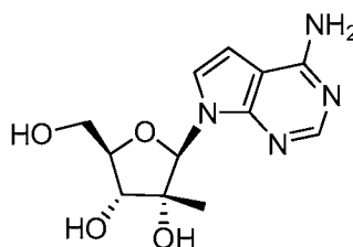
Compound A
