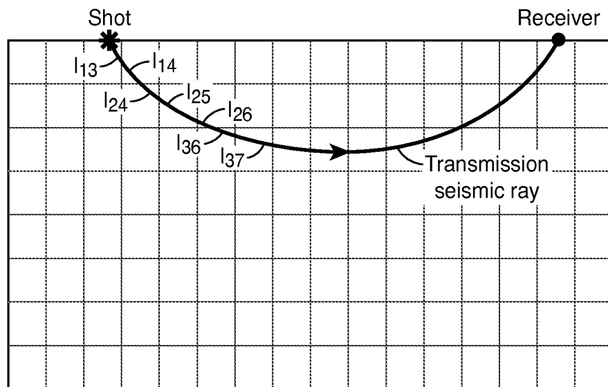
FIG. 2 (Prior Art)
