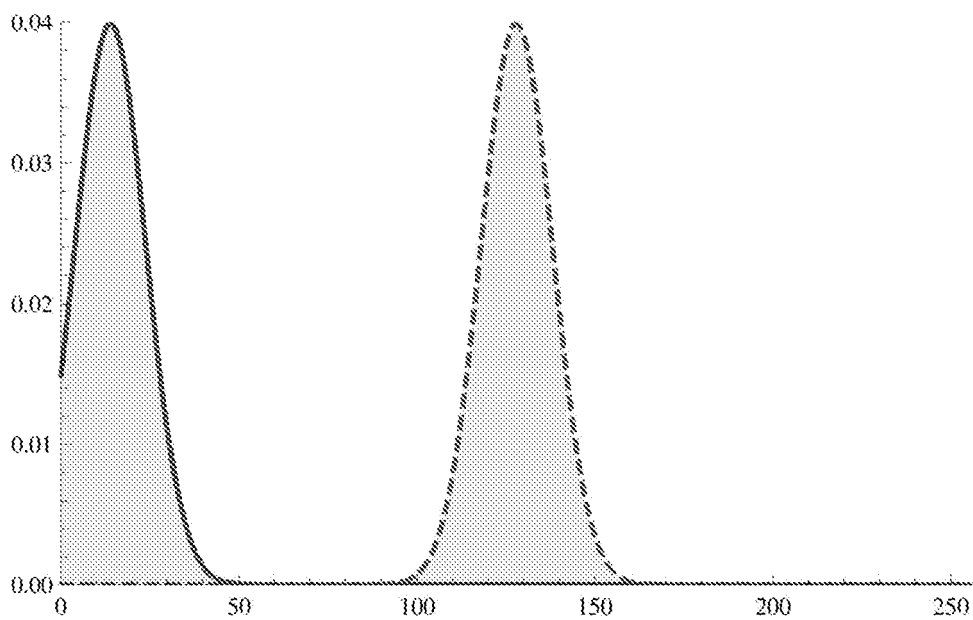
Fig. 5 Separated Error Distributions
