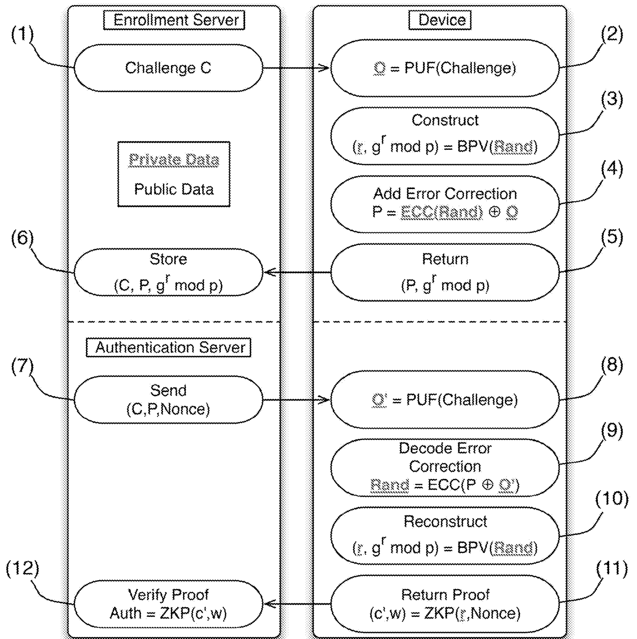
Fig. 1 Enrollment and Authentication Overview
