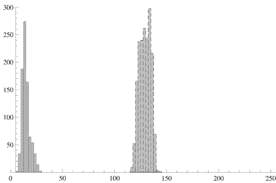
Fig. 6 True (Observed) Error Distributions
