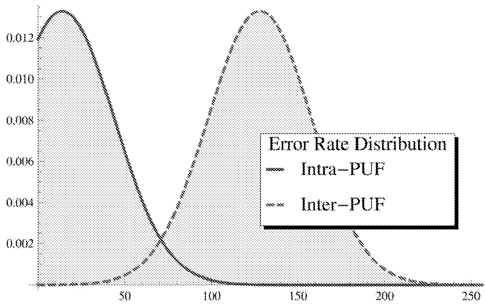
Fig. 4 Overlapping Error Distributions
