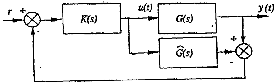
Internal Model Control (IMC) system configuration
