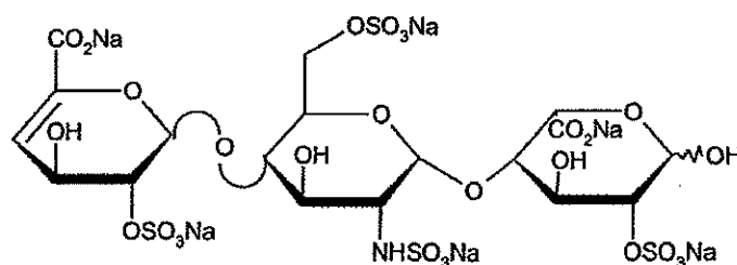
trisaccharide 1
