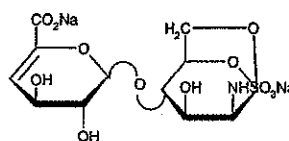
disaccharide 2
