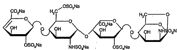
tetrasaccharide 1
