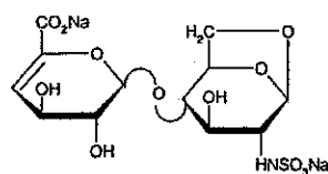
disaccharide 1
