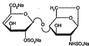
disaccharide 3
