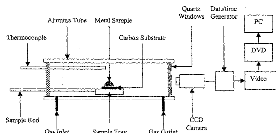
Figure 3 Schematic of horizontal tube furnace
