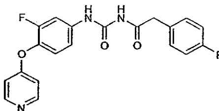
1-(3-Fluoro-4-(pyridin-4-yloxy)phenyl)-3-(2-(4-fluorophenyl)acetyl)urea
