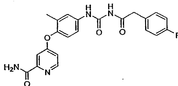
1-(4-(2-Carbamoylpyridin-4-yloxy)-3-methylphenyl)-3-(2-(4-fluorophenyl)acetyl)urea
