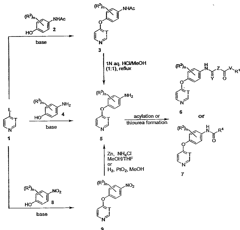
SCHEME 1
