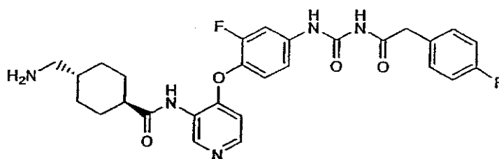
1-(4-(3-((1R,4R)-4-(Aminomethyl)cyclohexanecarboxamido)pyridin-4-yloxy)-3-fluorophenyl)-3-(2-(4-fluorophenyl)acetyl)urea
