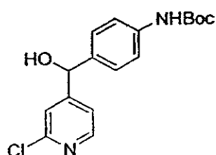
1-(4-((2-(3-(Dimethylamino)propylamino)pyridin-4-yl)(hydroxy)methyl)phenyl)- 3-(2-(4-fluorophenyl)acetyl)urea
