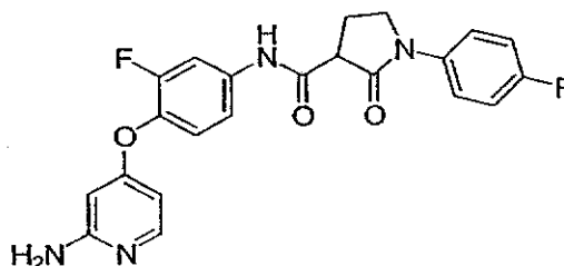
15 N -(4-(2-Aminopyridin-4-yloxy)-3-fluorophenyl)-1-(4-fluorophenyl)-2-oxopyrrolidine-3-carboxamide
