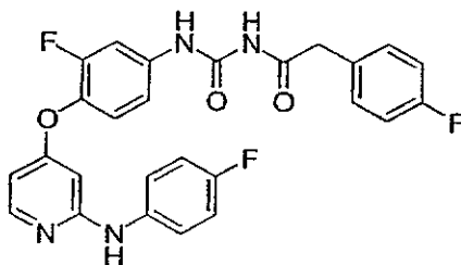
1-(3-Fluoro-4-(2-(4-fluorophenylamino)pyridin-4-yloxy)phenyl)-3-(2-(4-fluorophenyl)acetyl)urea
