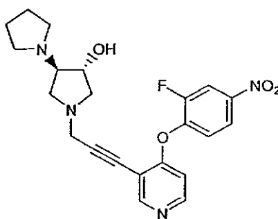
A) (3R,4R)-1-(3-(4-(2-Fluoro-4-nitrophenoxy)pyridin-3-yl)prop-2-ynyl)-4-(pyrrolidin-1-yl)pyrrolidin-3-ol
