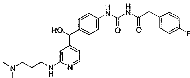
1-(4-((2-(3-(Dimethylamino)propylamino)pyridin-4-yl)(hydroxy)methyl)phenyl)- 3-(2-(4-fluorophenyl)acetyl)urea
