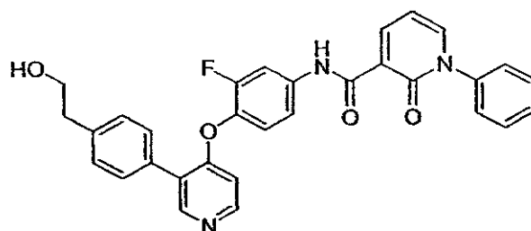
N -(3-Fluoro-4-(3-(4-(2-hydroxyethyl)phenyl)pyridin-4-yloxy)phenyl)-2-oxo-1-phenyl-1,2-dihydropyridine-3-carboxamide
