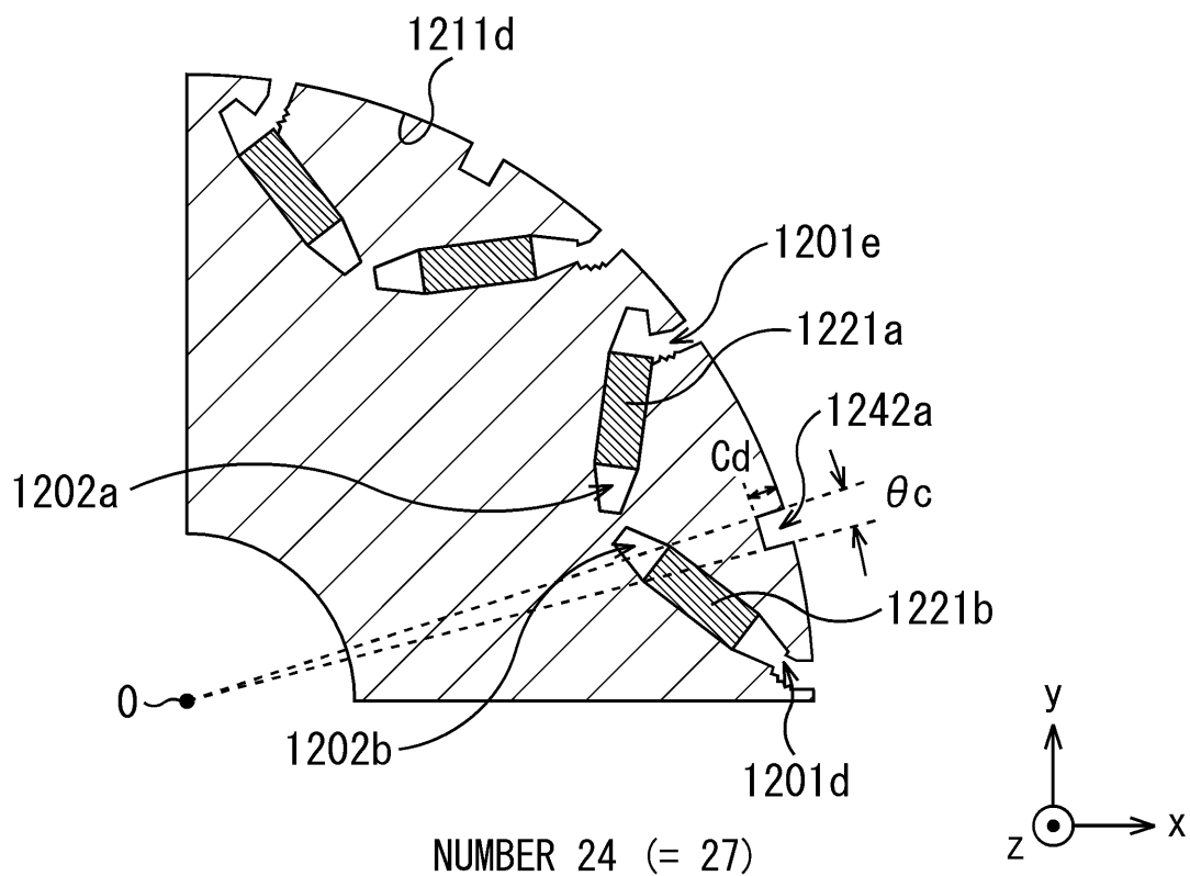
FIG. 12D
