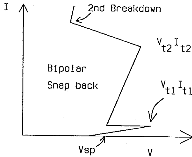
FIG. 5C - Prior Art
