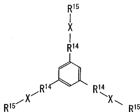
Structural formula (8)
