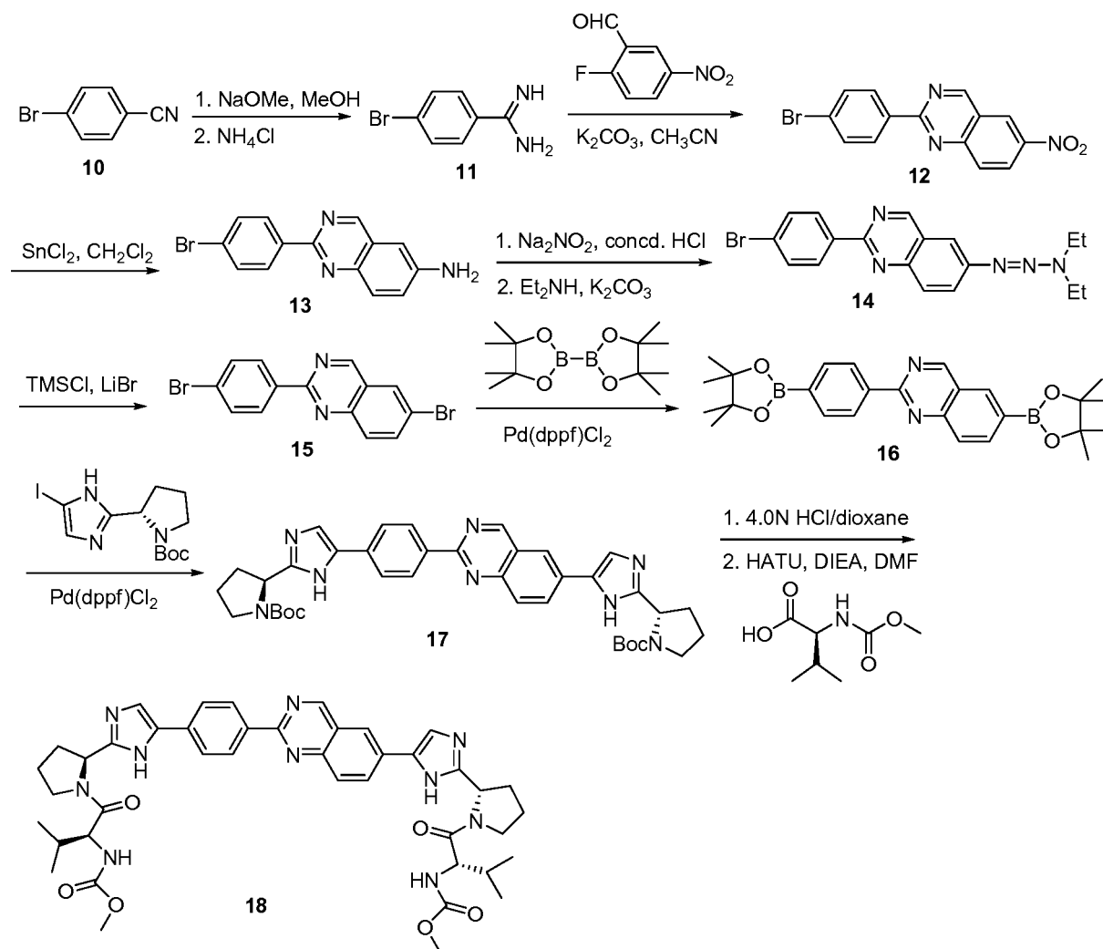
Scheme 3-3
