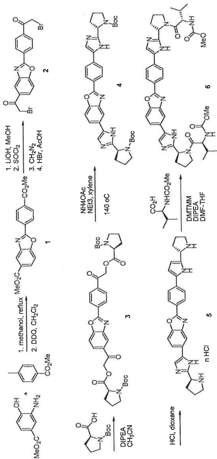
Scheme 9-3
