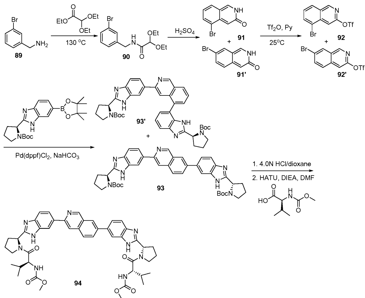
Scheme 7-2
