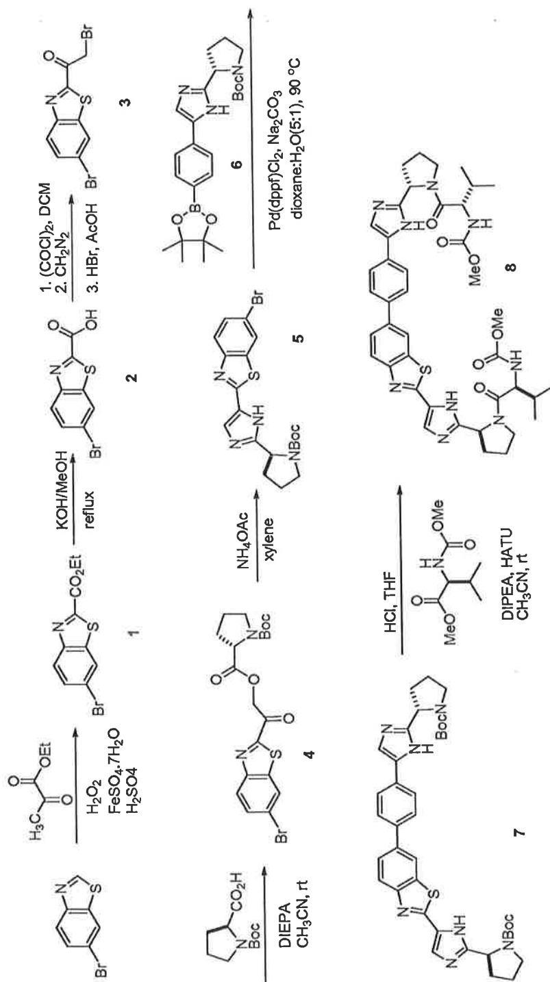
Scheme 12-9
