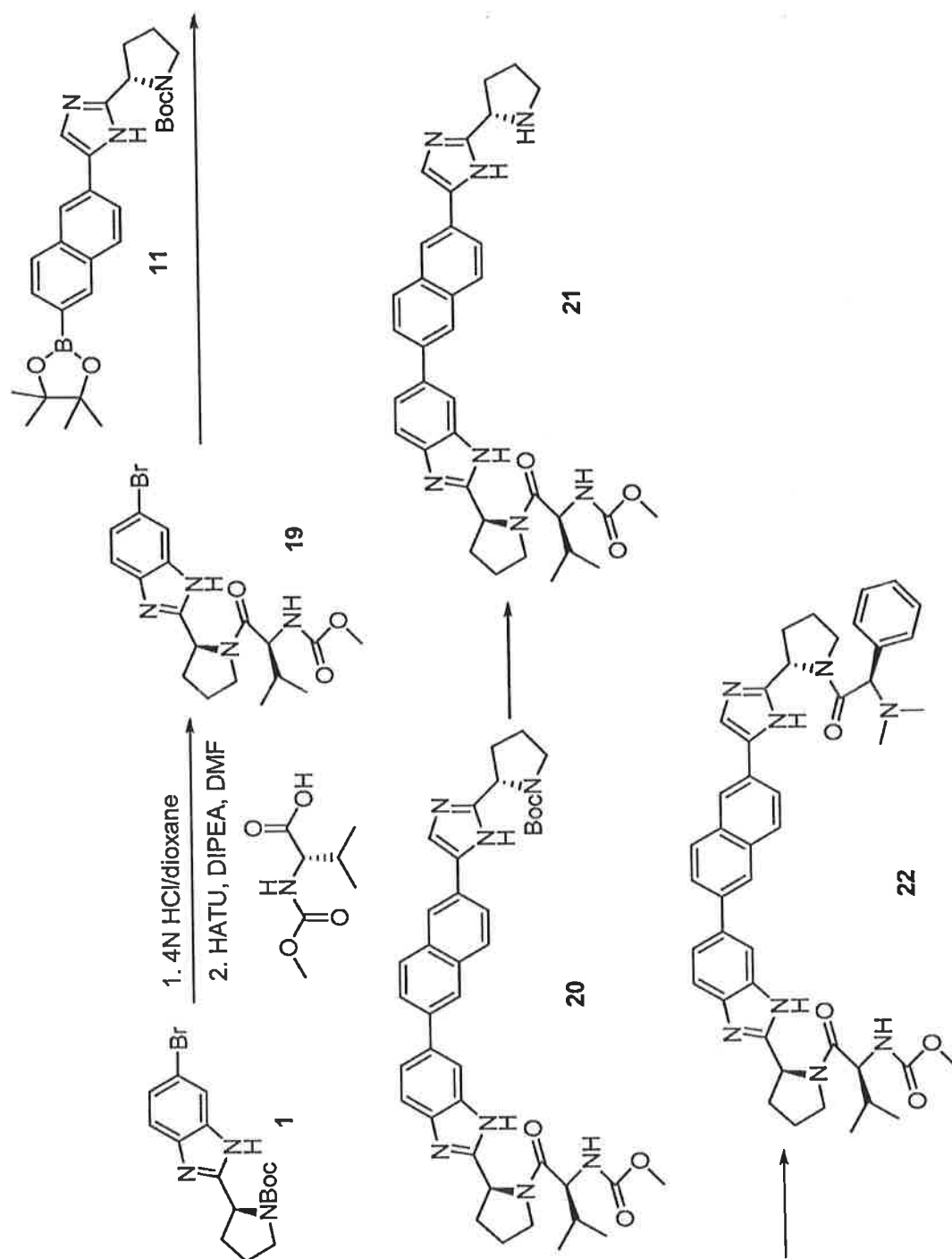
Scheme 2-3
