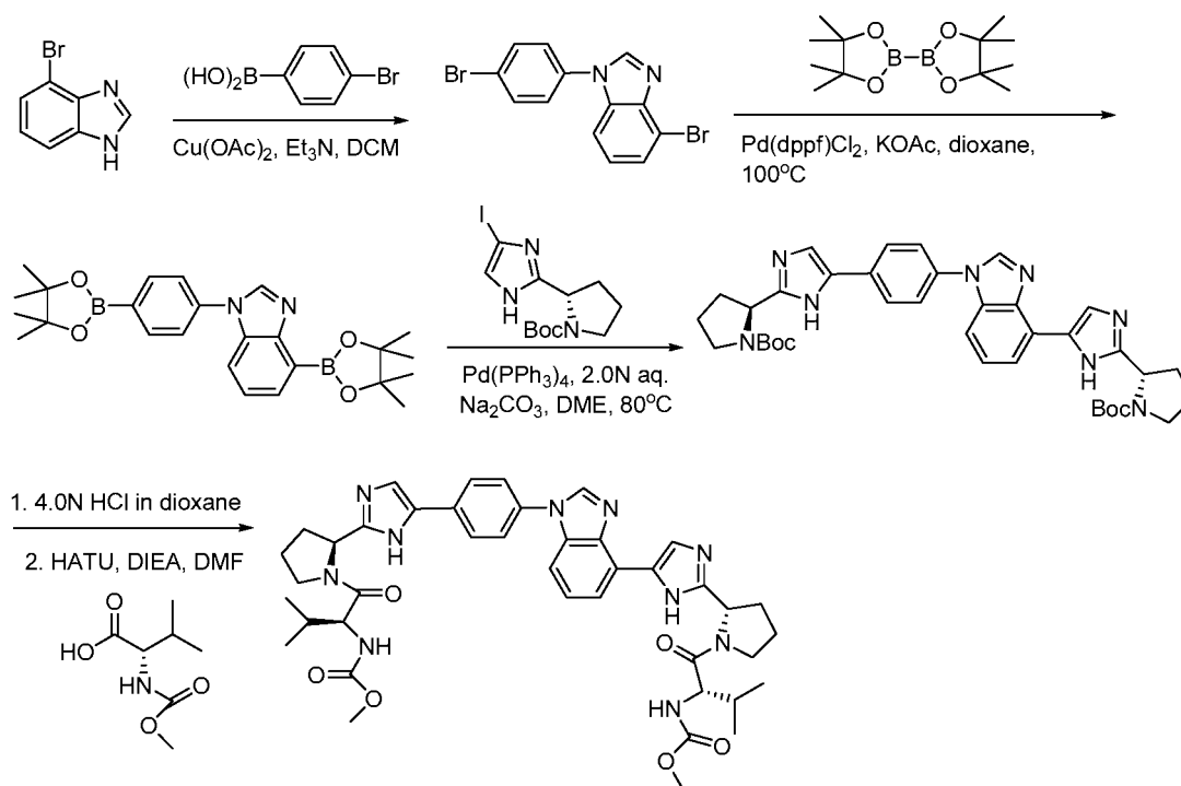
Scheme 12-4
