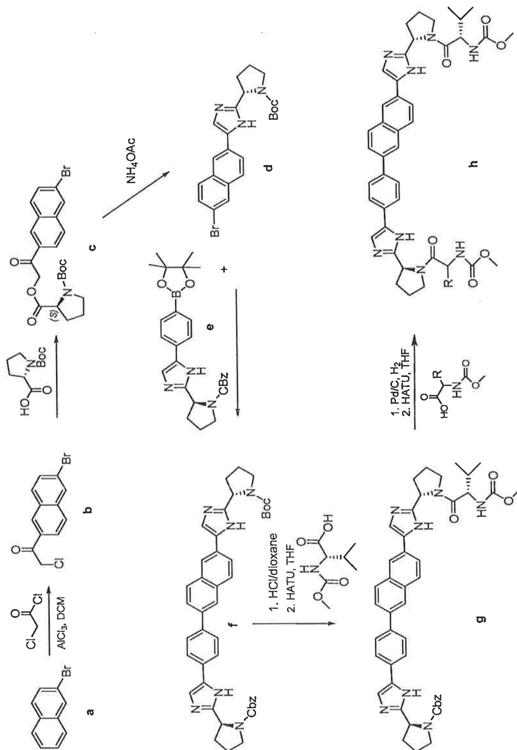
Scheme 1-1
