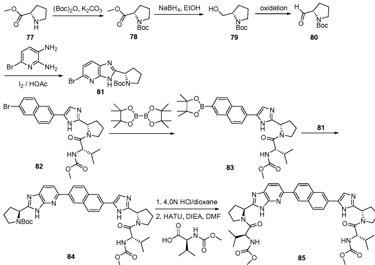
Scheme 6-2
