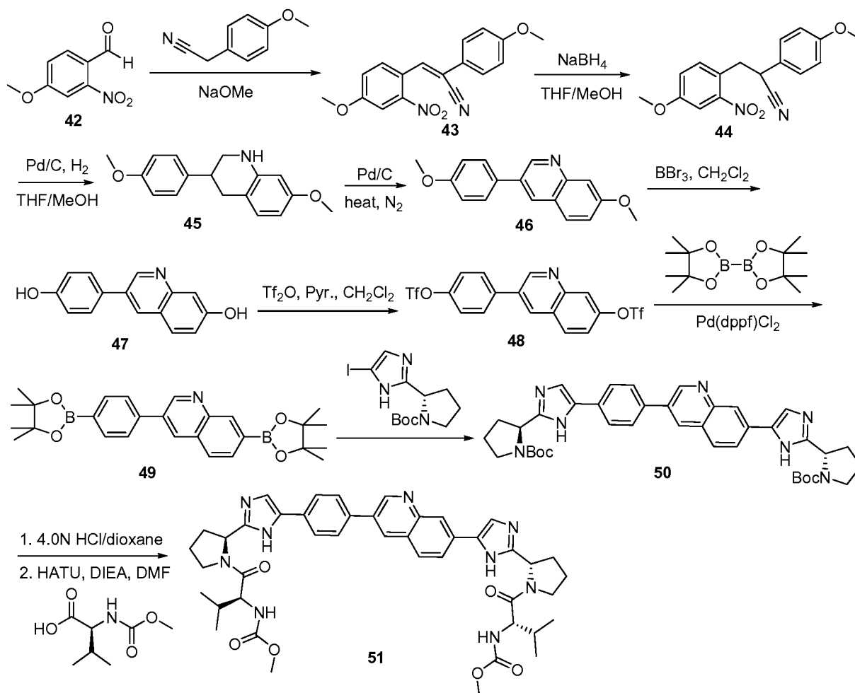
Scheme 3-6
