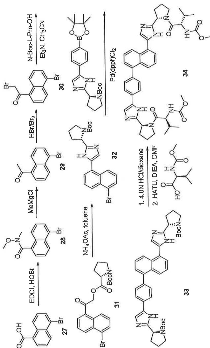
Scheme 4-1
