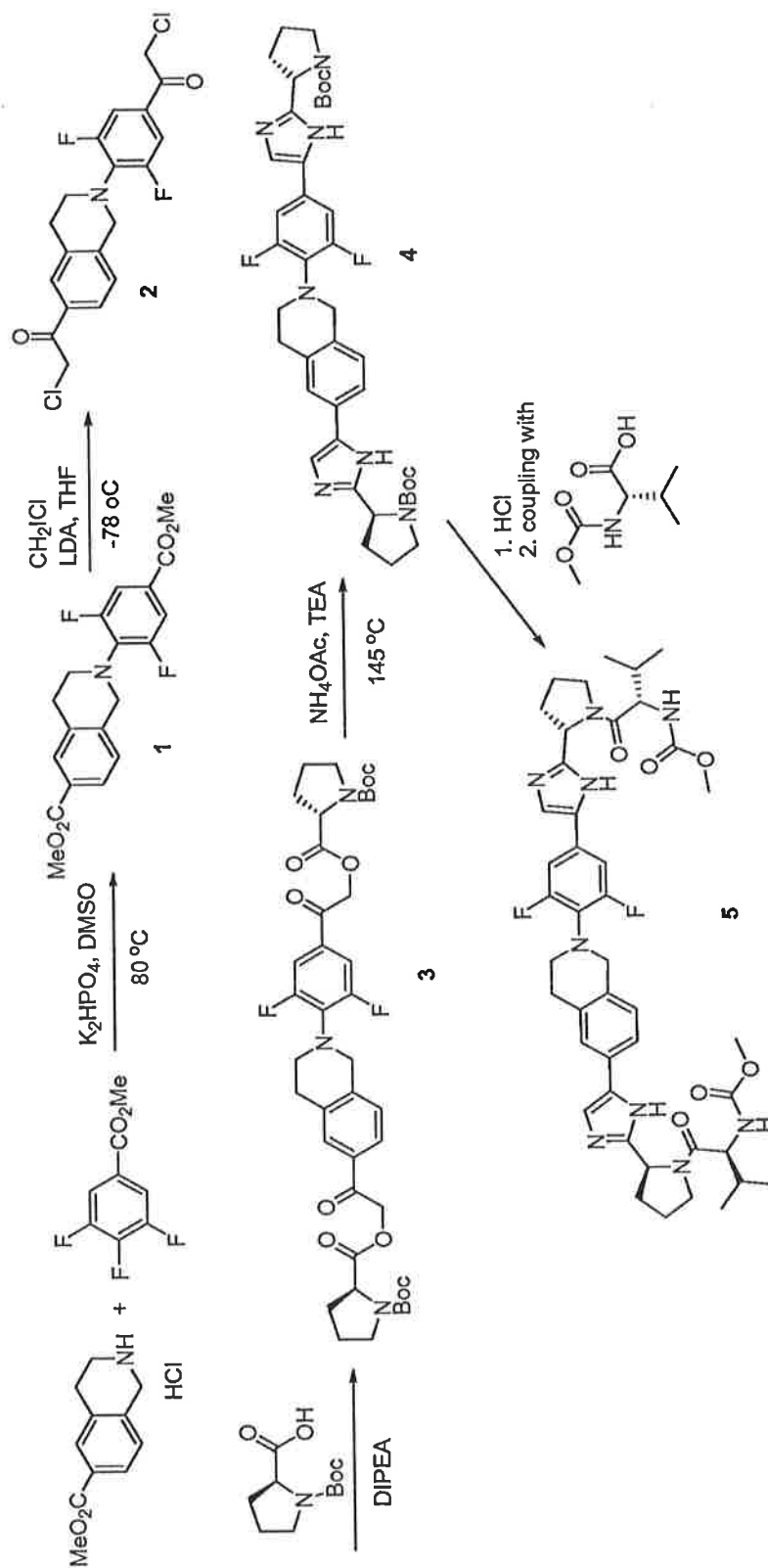
Scheme 10-1
