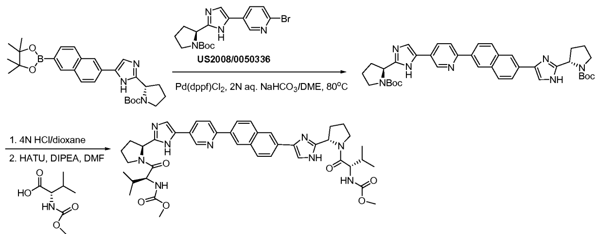
Scheme 12-7
