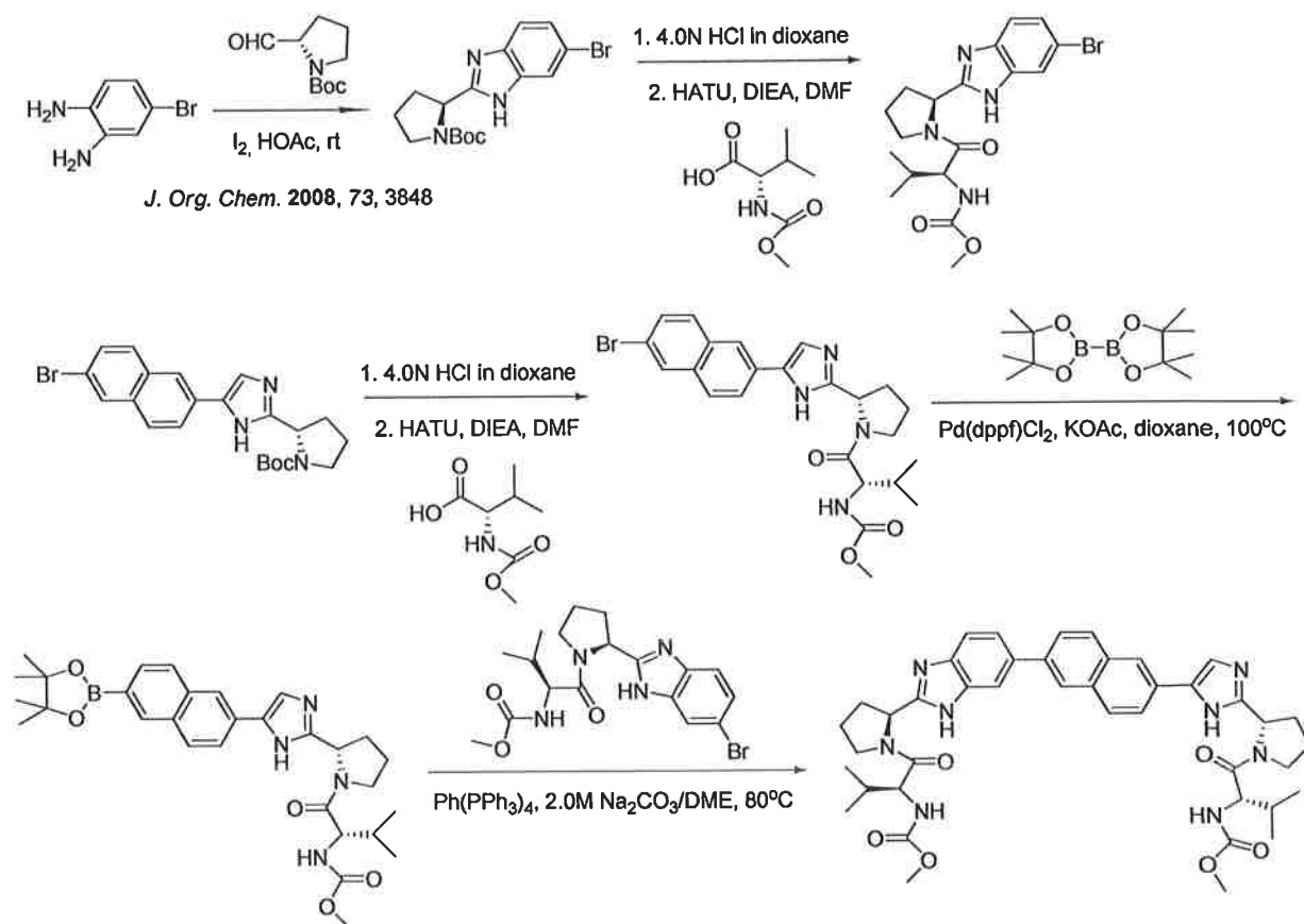
Scheme 2-1-1
