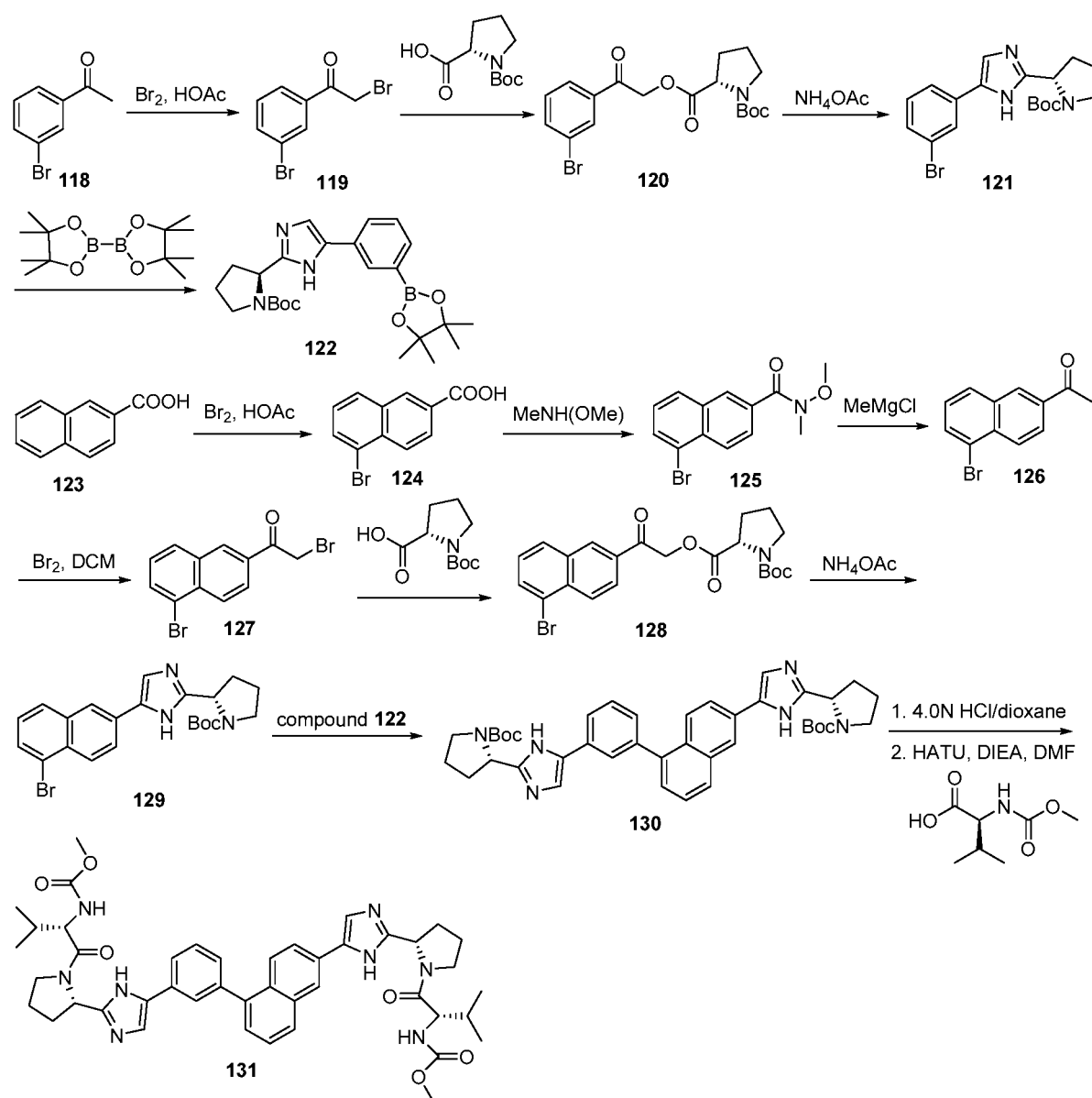
Scheme 8-1
