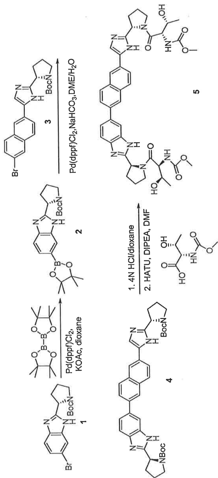
Scheme 2-1
