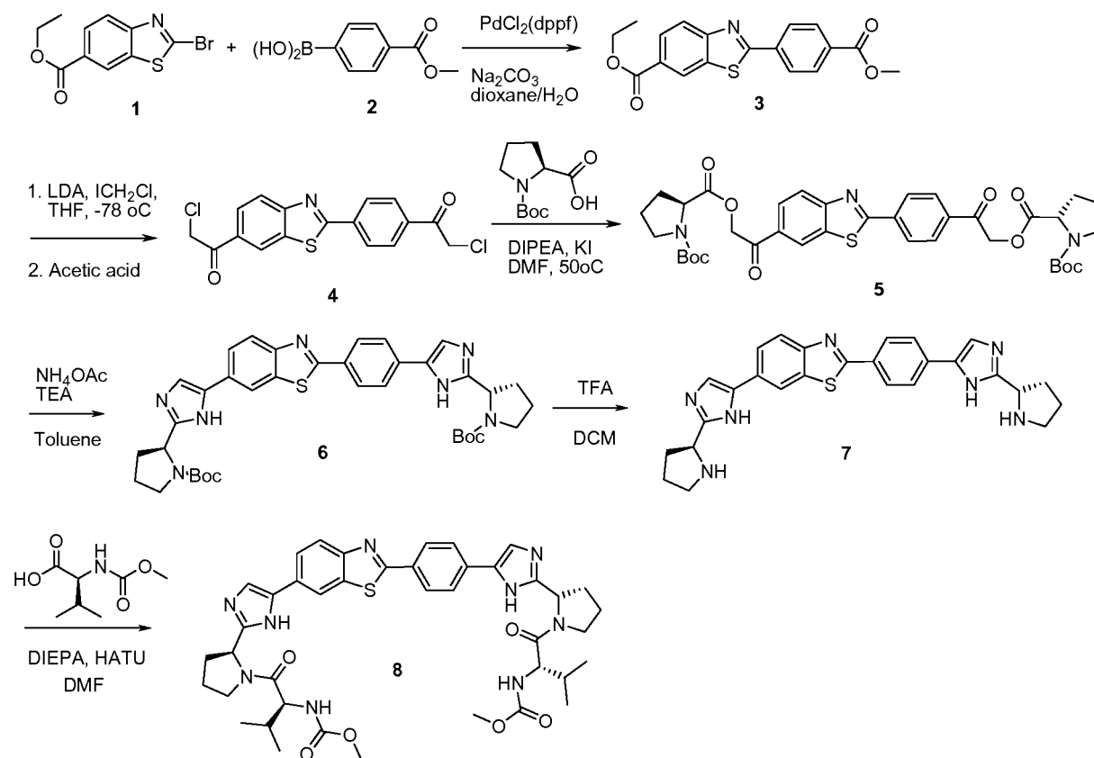
Scheme 9-1
