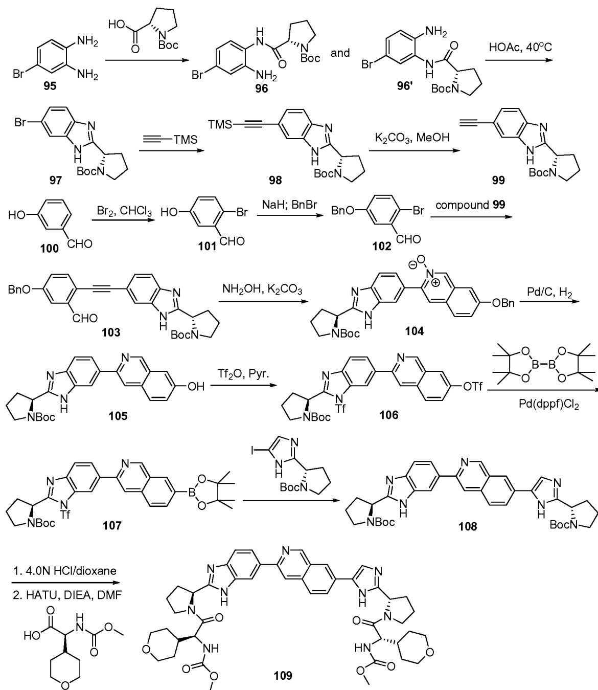
Scheme 6-3
