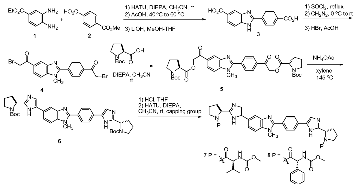
Scheme 9-2
