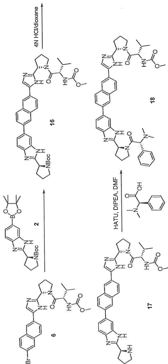
Scheme 2-2
