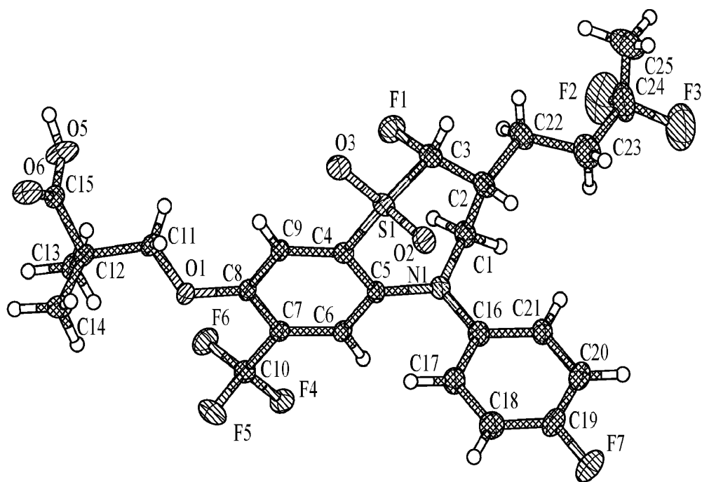
FIG. 1 The ORTEP plot for Example 10b.
