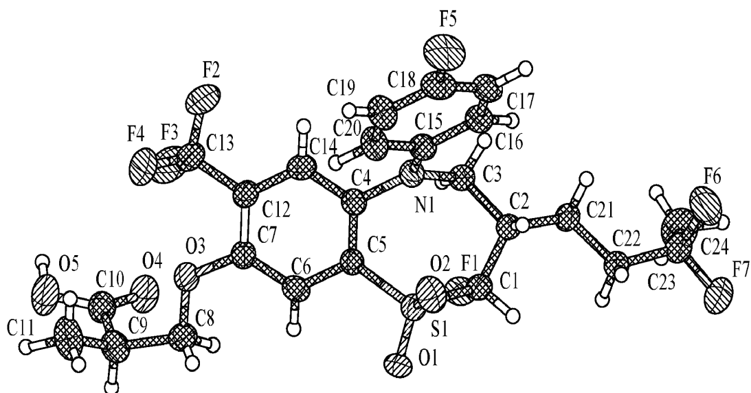
FIG. 2 The ORTEP plot for Example 11a.
