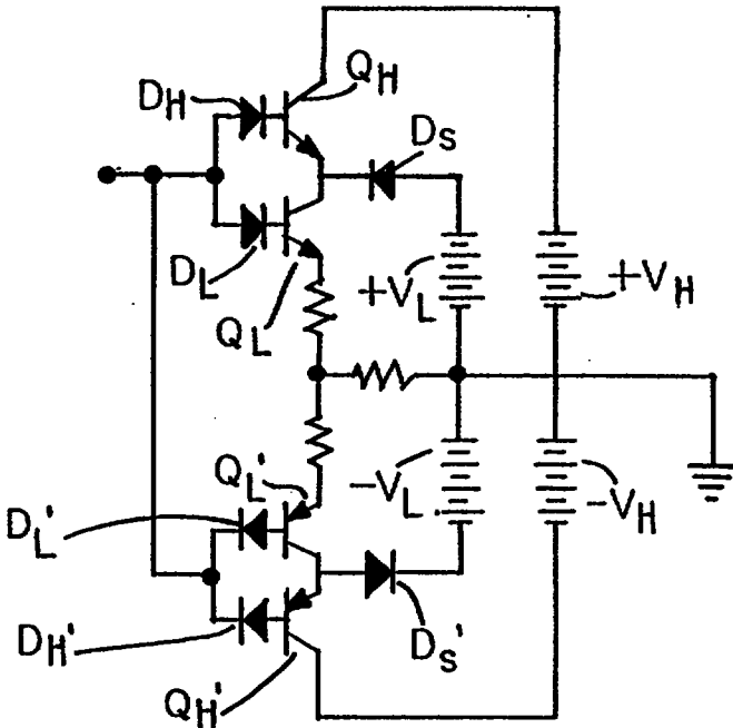
Fig. 3. (PRIOR ART)
