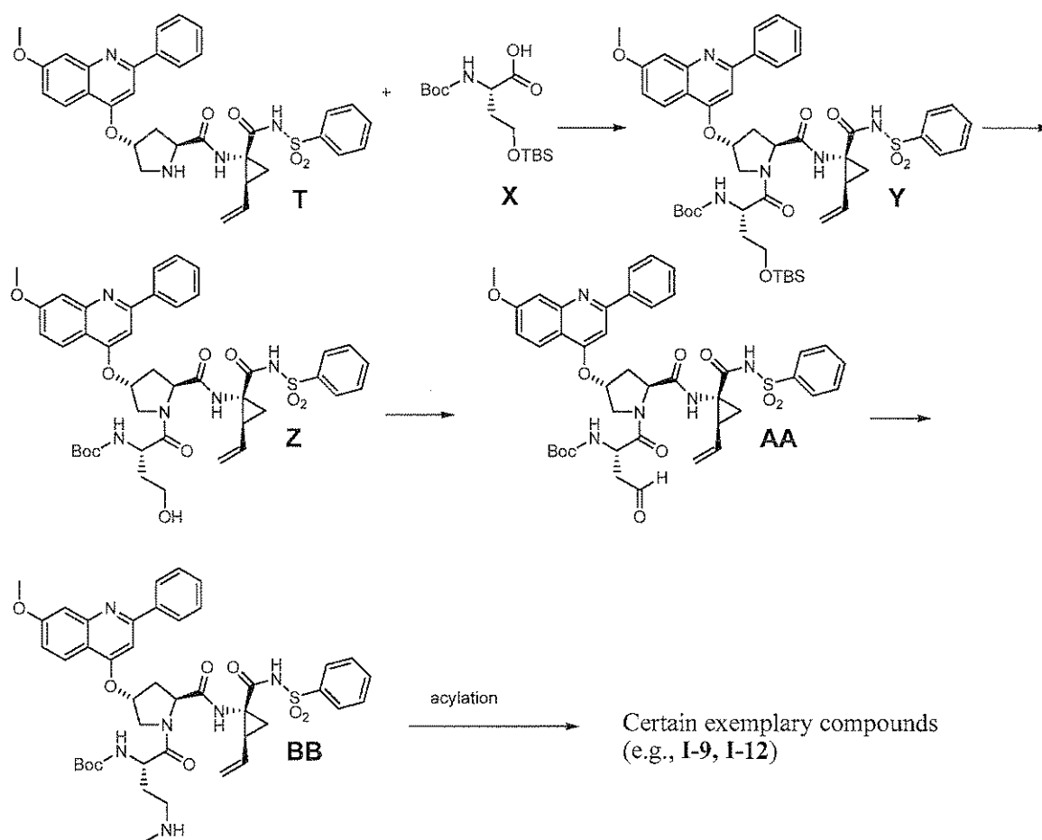
Scheme 4
