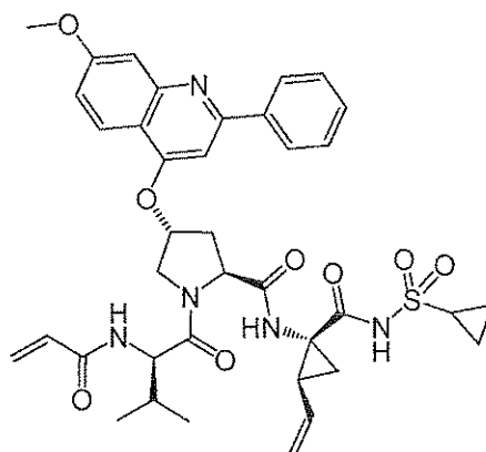
Compound I-56
