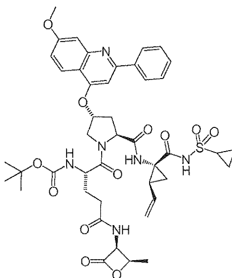
Compound I-67
