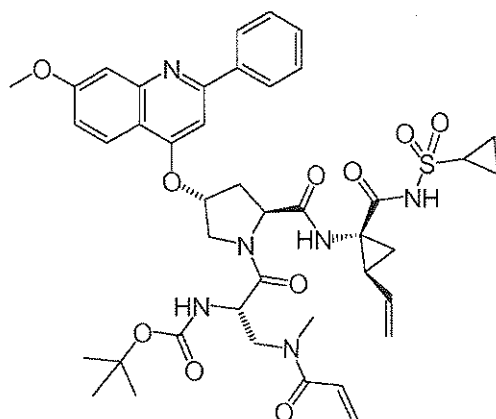
Compound (I-52)
