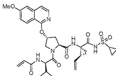
Compound I-101
