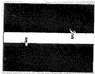
Red-Al
