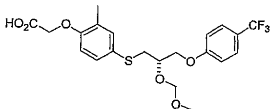
Compound 23
