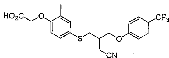
Compound 10
