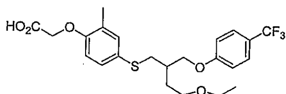
Compound 37
