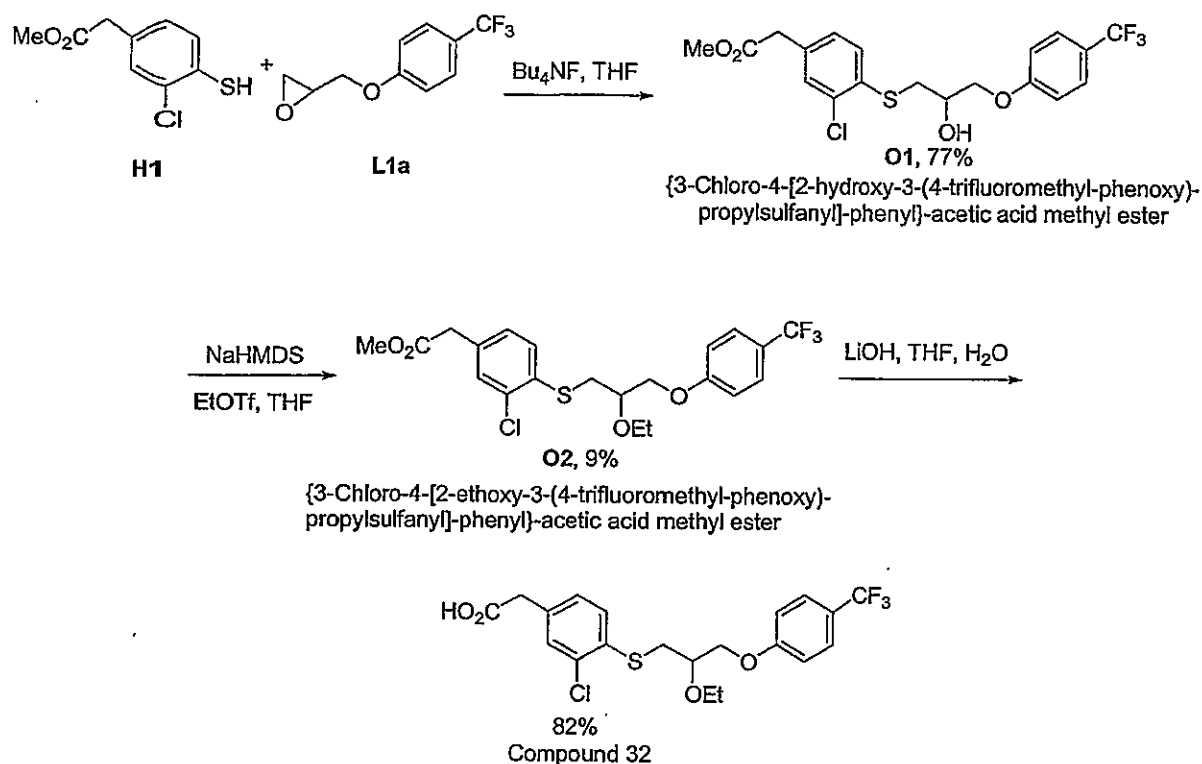
Scheme O
