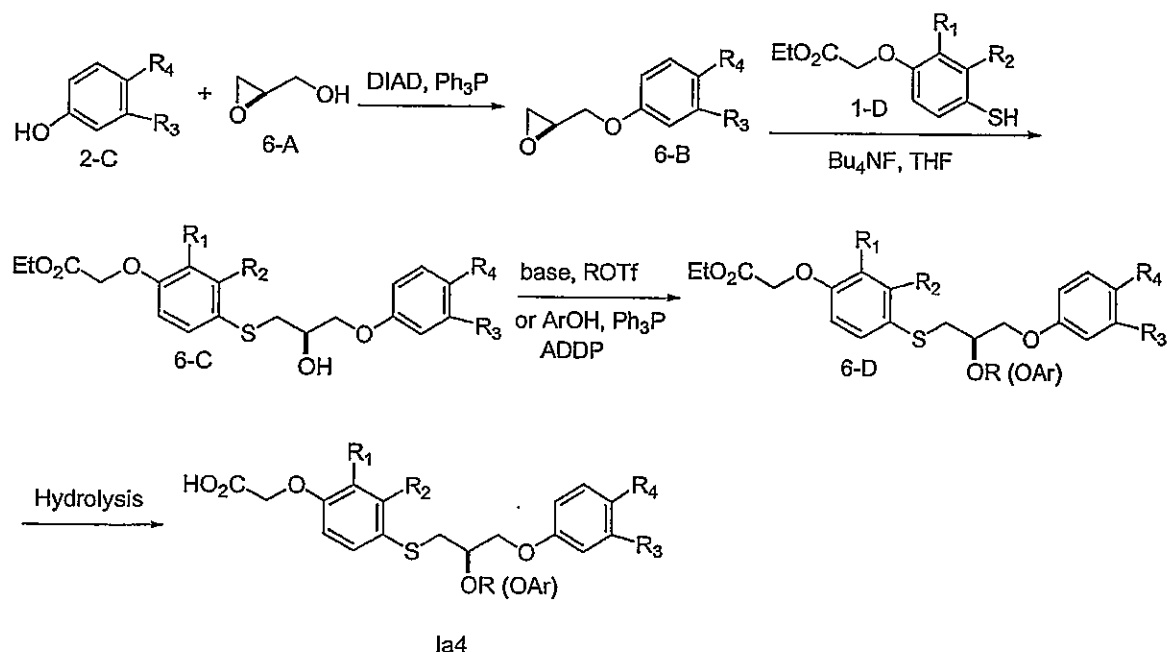
Scheme 6. Synthesis of Compound 1a4
