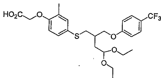
Compound 36
