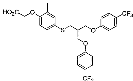
Compound 34
