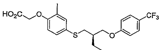
Compound 2 :
