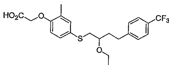
Compound 38
