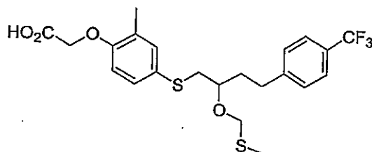
Compound 39
