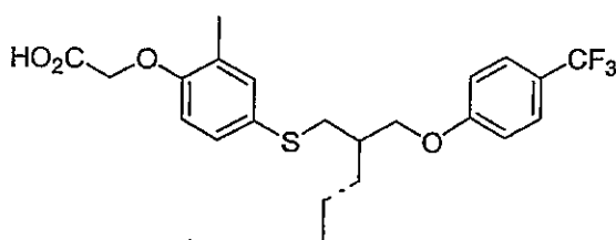
Compound 5
