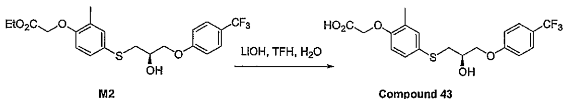
Scheme T
