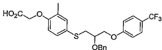
Compound 28
