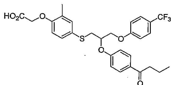
Compound 30
