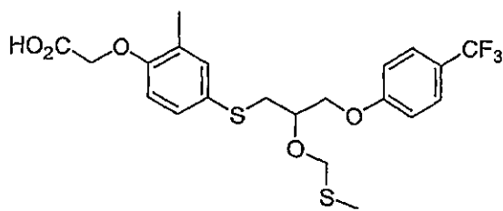
Compound 25
