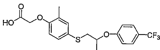
Compound 7
