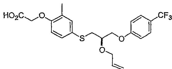
Compound 20
