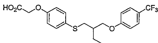
Compound 4
