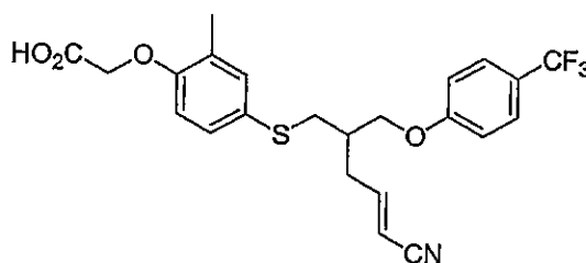
Compound 12
