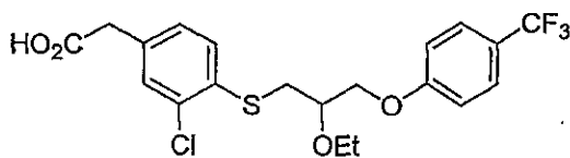
Compound 32.
