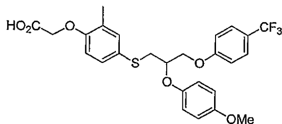
Compound 29
