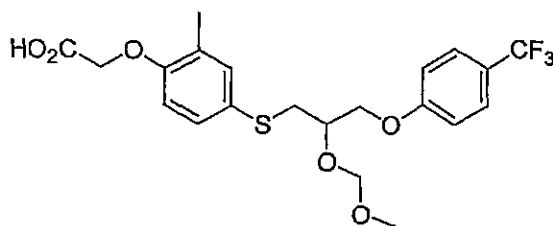
Compound 24
