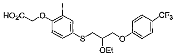
Compound 17
