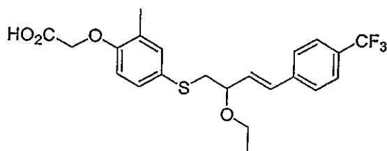
Compound 42
