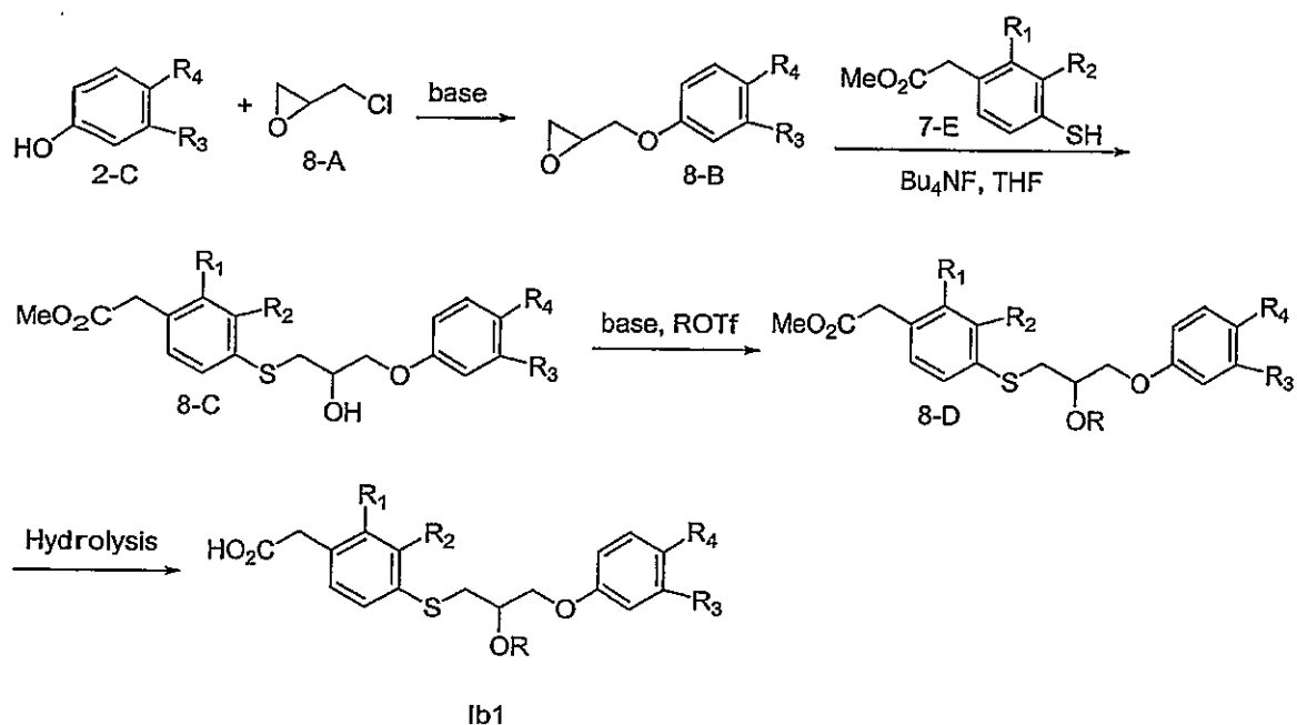
Scheme 8. Synthesis of Compound Ib1
