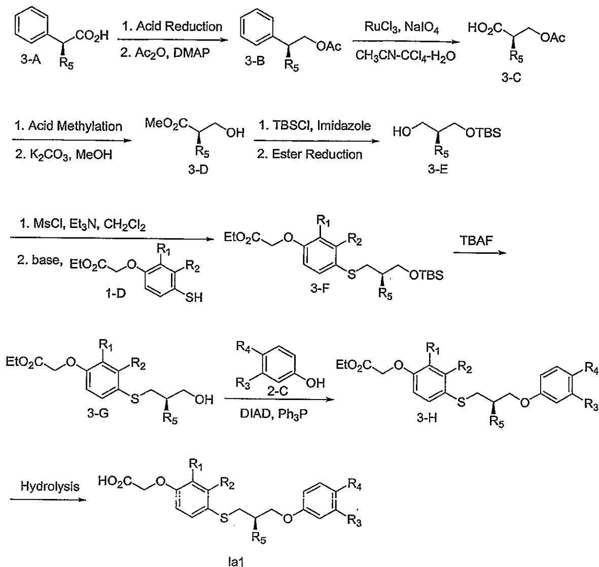
Scheme 3. Synthesis of Compound Ia1
