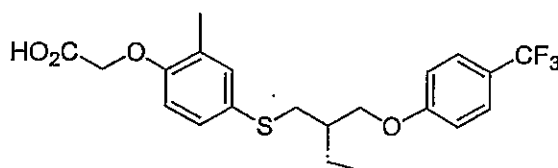
Compound 3
