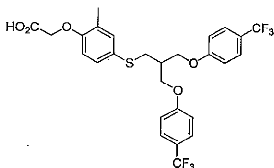
Compound 34
