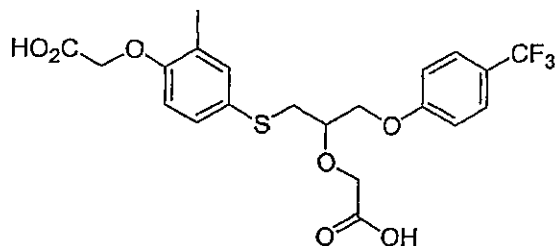
Compound 26
