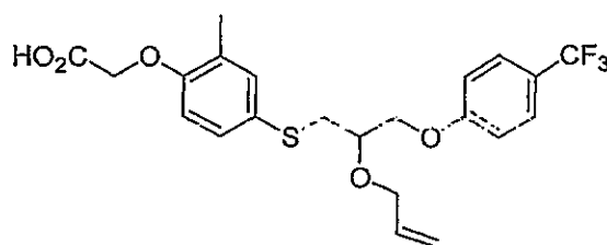
Compound 21
