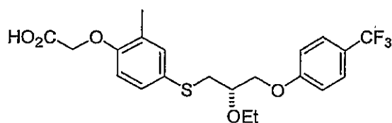
Compound 16
