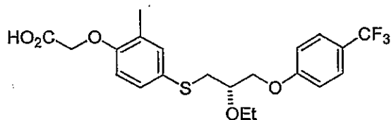
Compound 16
