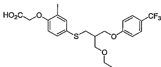
Compound 33
