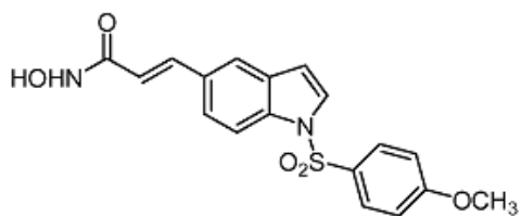
Compound 4
