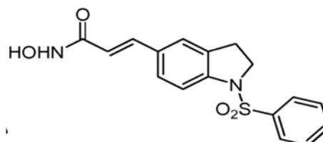
Compound 12
