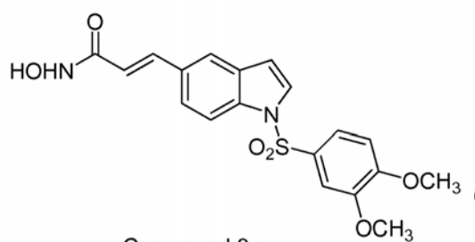
Compound 8
