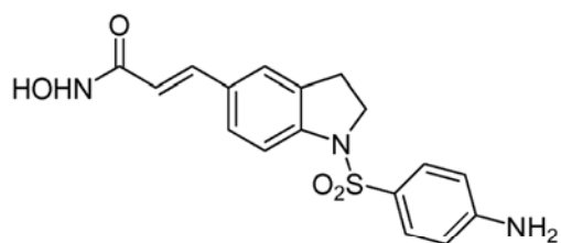
Compound 16
