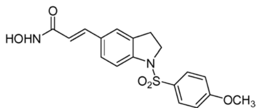
Compound 13
