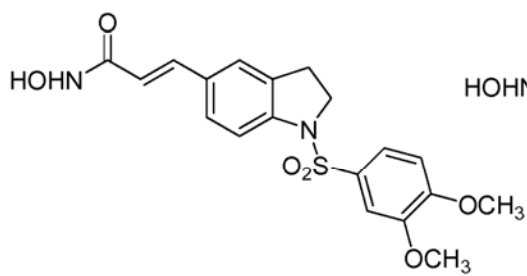
Compound 17
