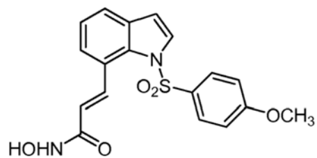
Compound 28
