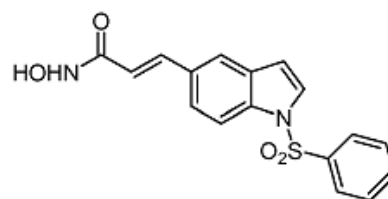
Compound 3
