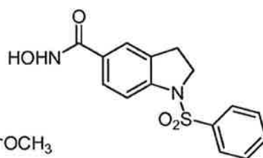
Compound 18
