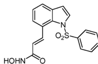
Compound 22
