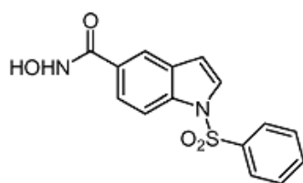
Compound 1
