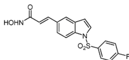
Compound 5
