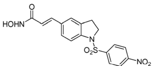
Compound 15
