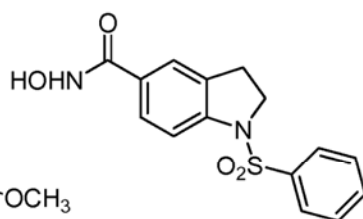
Compound 18
