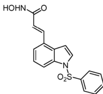
Compound 21
