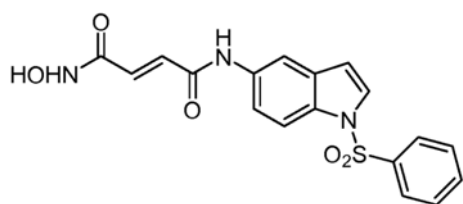
Compound 27
