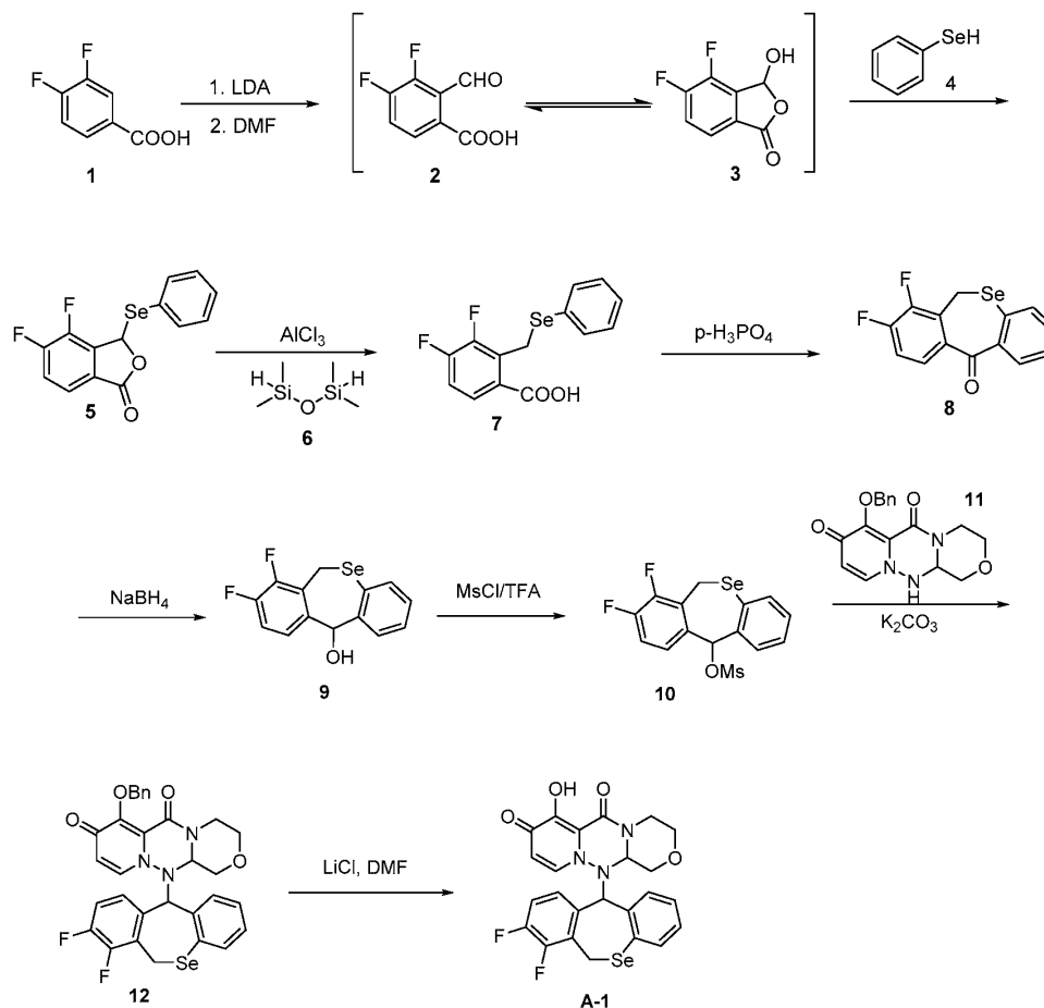
Scheme 1. Synthesis of A-1
