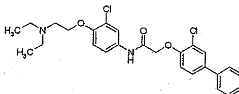
2-(3-chloro-biphenyl-4-yloxy)-N-[3-chloro-4-(2-diethylamino-ethoxy)-phenyl]-acetamide
