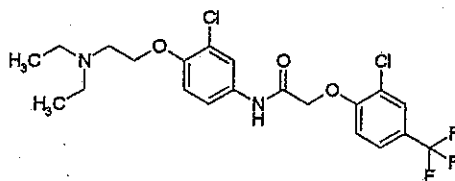
N-[3-chloro-4-(2-diethylamino-ethoxy)-phenyl]-2-(2-chloro-4-trifluoromethyl-phenoxy)-acetamide
