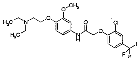
2-(2-chloro-4-trifluoromethyl-phenoxy)-N-[4-(2-diethylamino-ethoxy)-3-methoxy-phenyl]-acetamide
