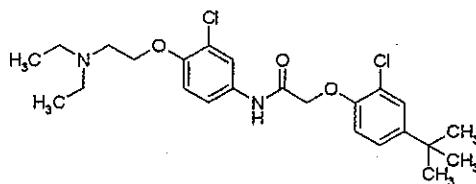
2-(4-tert-butyl-2-chloro-phenoxy)-N-[3-chloro-4-(2-diethylamino-ethoxy)-phenyl]-acetamide
