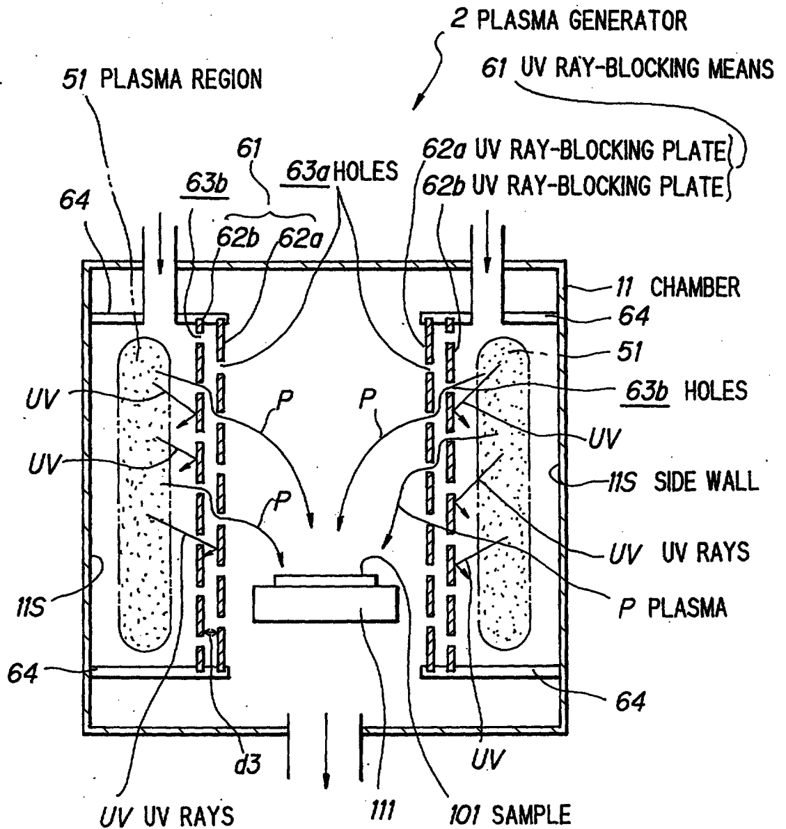
SCHEMATIC CROSS SECTION OF SECOND EXAMPLE OF PLASMA GENERATOR
