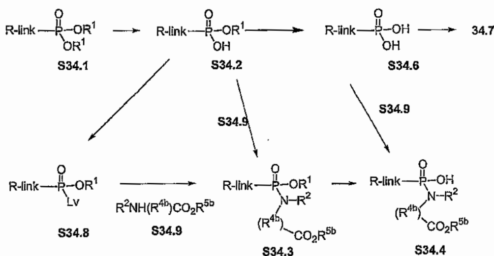
Scheme 34
