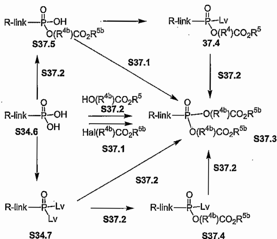
Scheme 37
