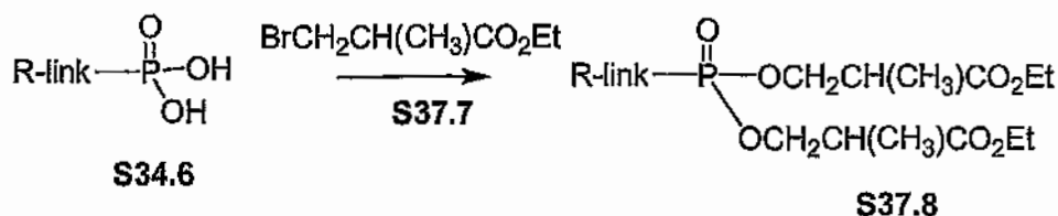
Scheme 37 Example 2
