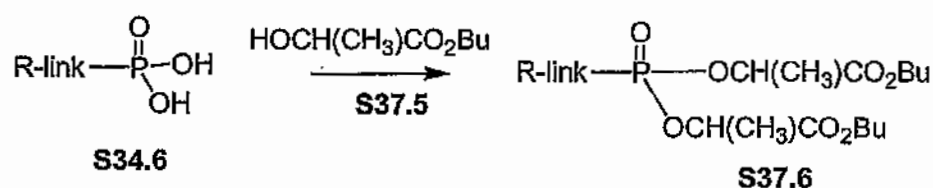
Scheme 37 Example 2
