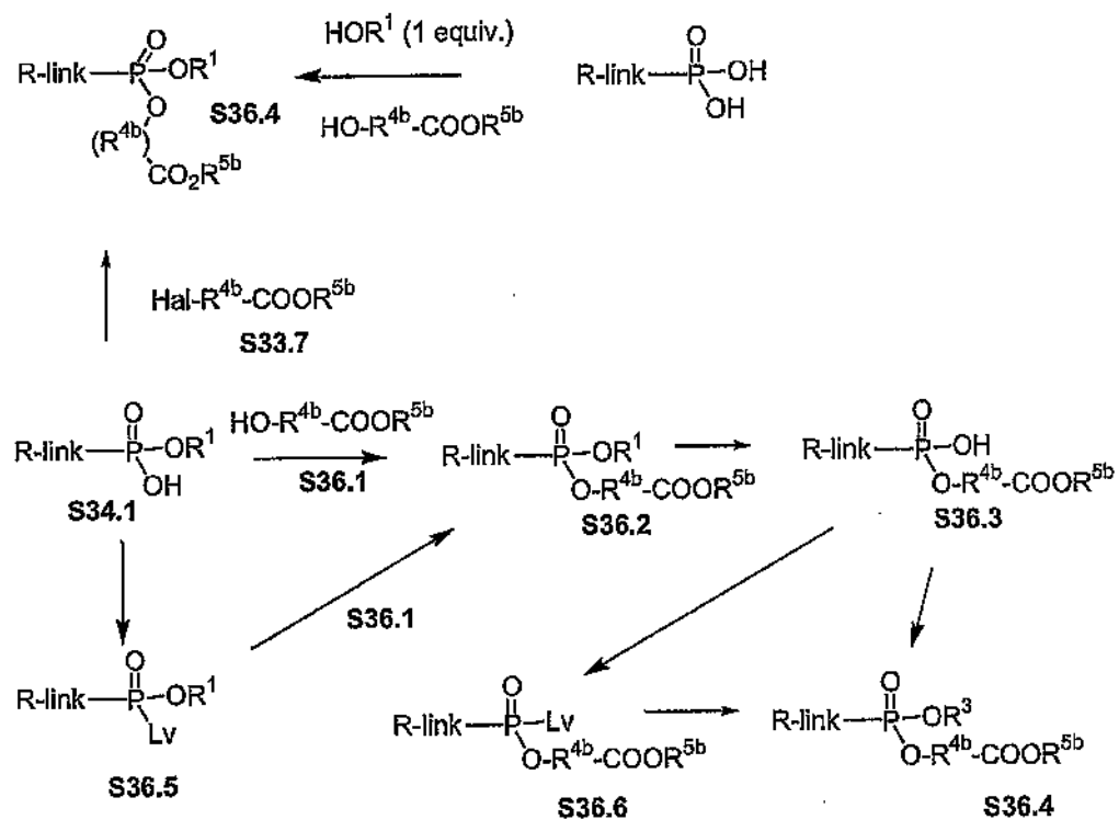
Scheme 36
