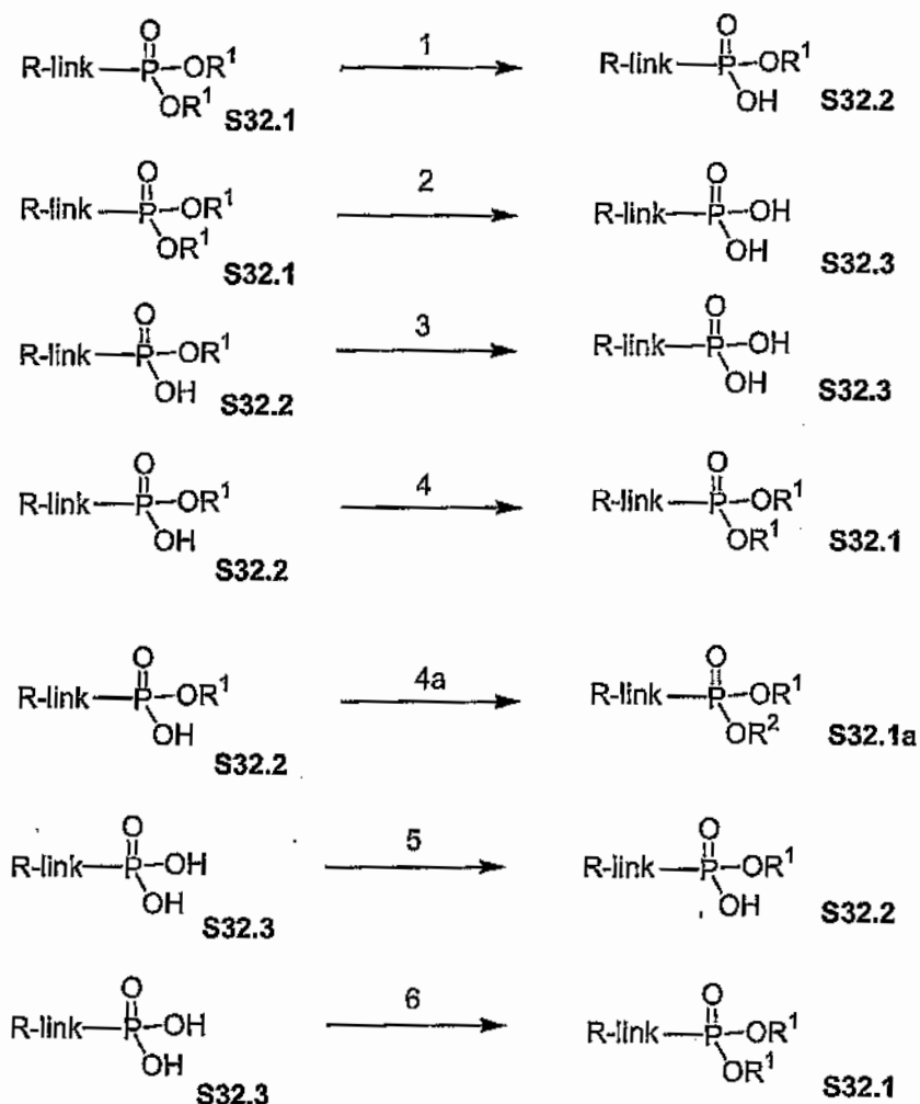
Scheme 32
