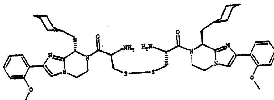
COMPOUND 41
