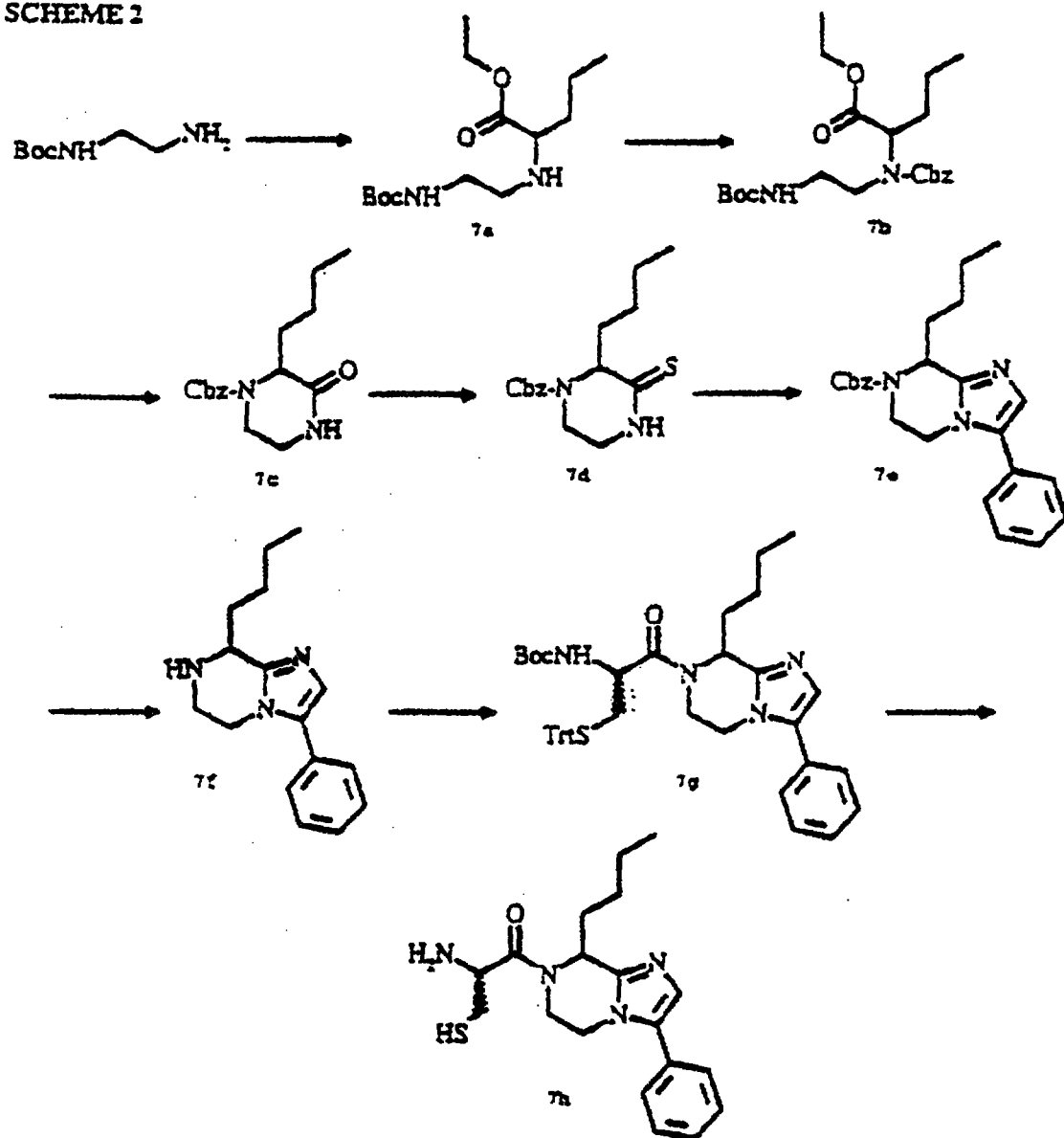
SCHEME 2
