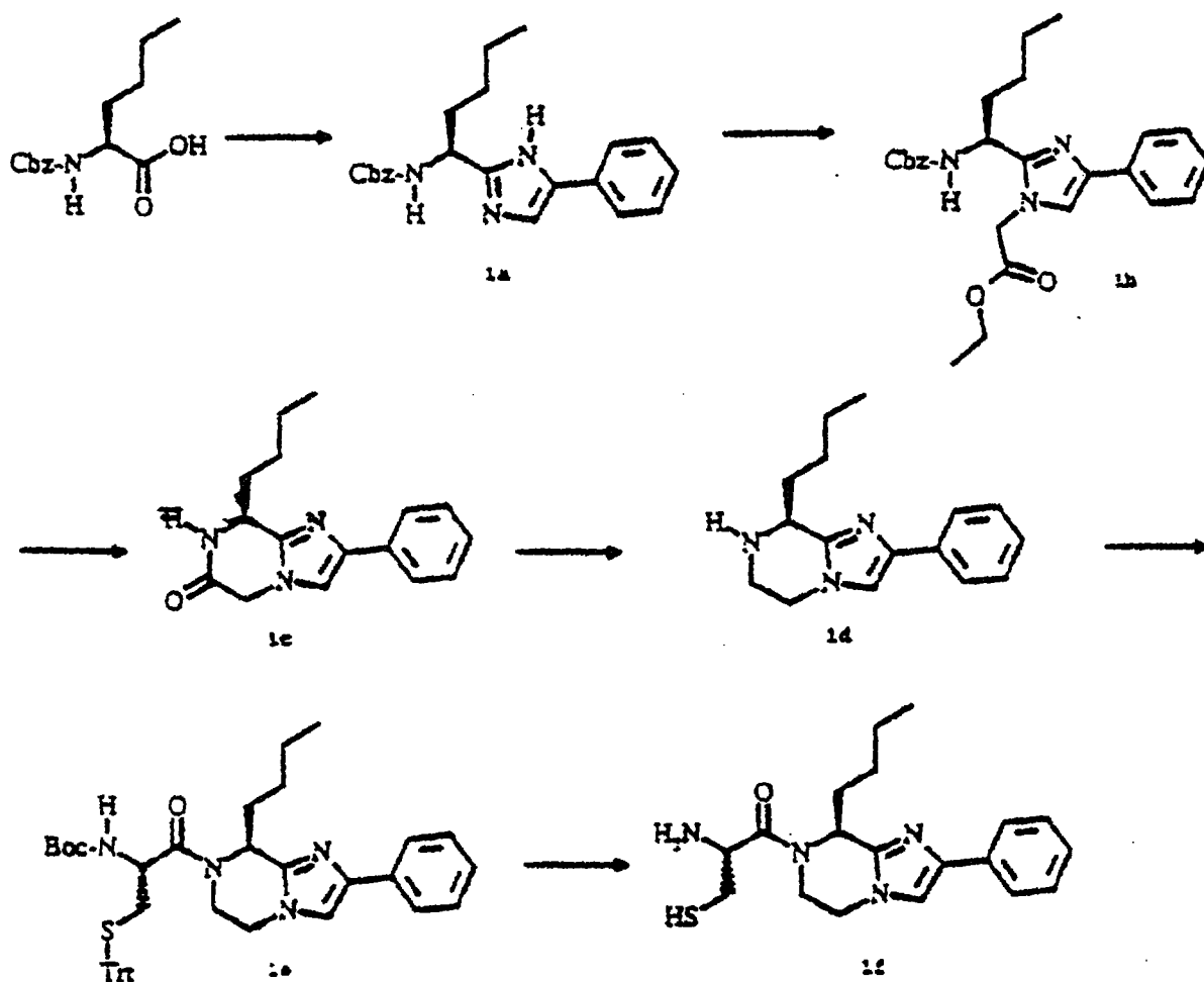
SCHEME 1
