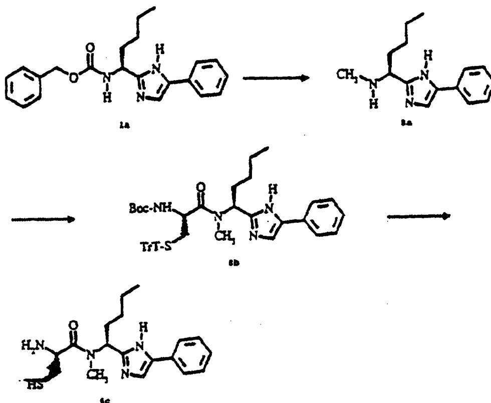
SCHEME 3
