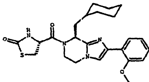
COMPOUND 62
