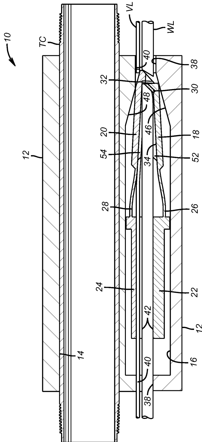
FIG. 4 (PRIOR ART)
