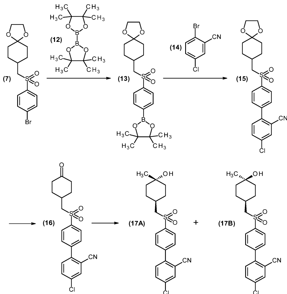
Scheme 4
