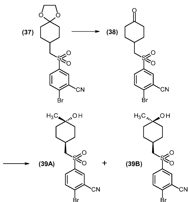
Scheme 11
