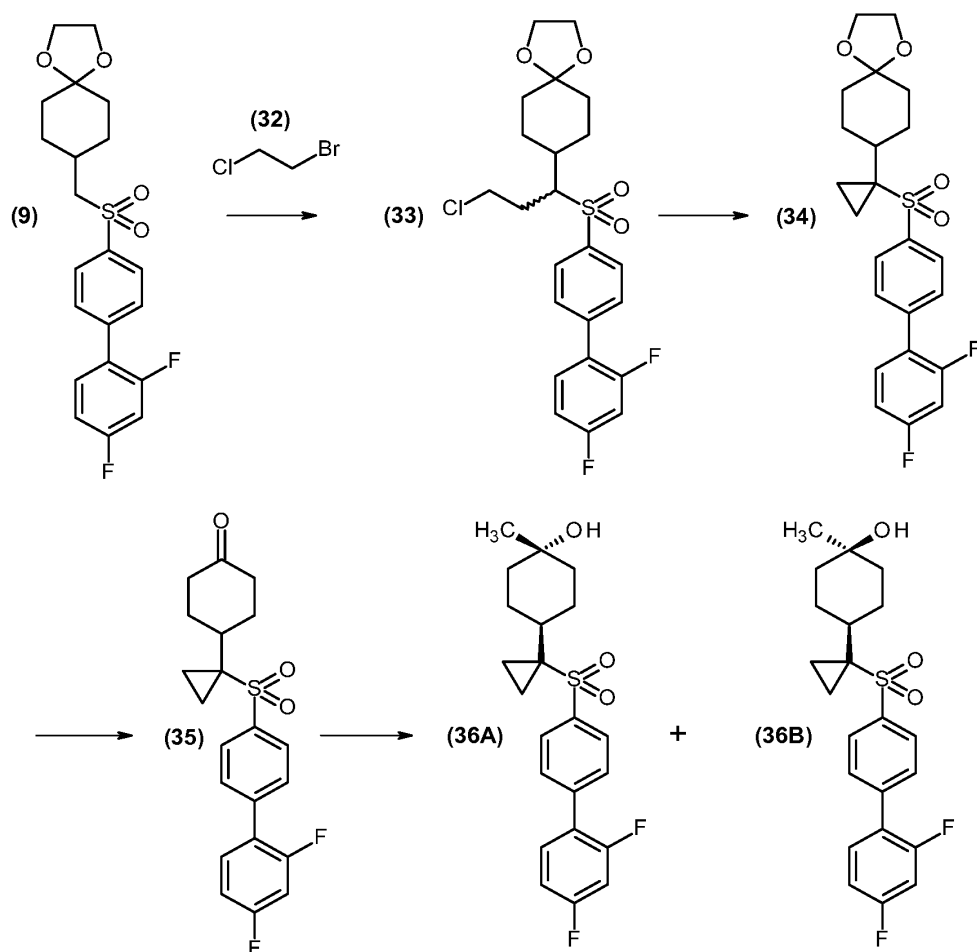
Scheme 10
