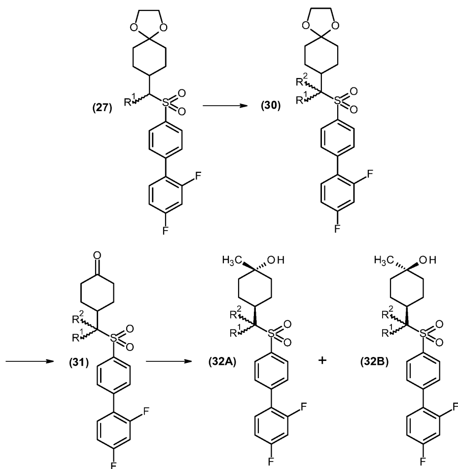
Scheme 9
